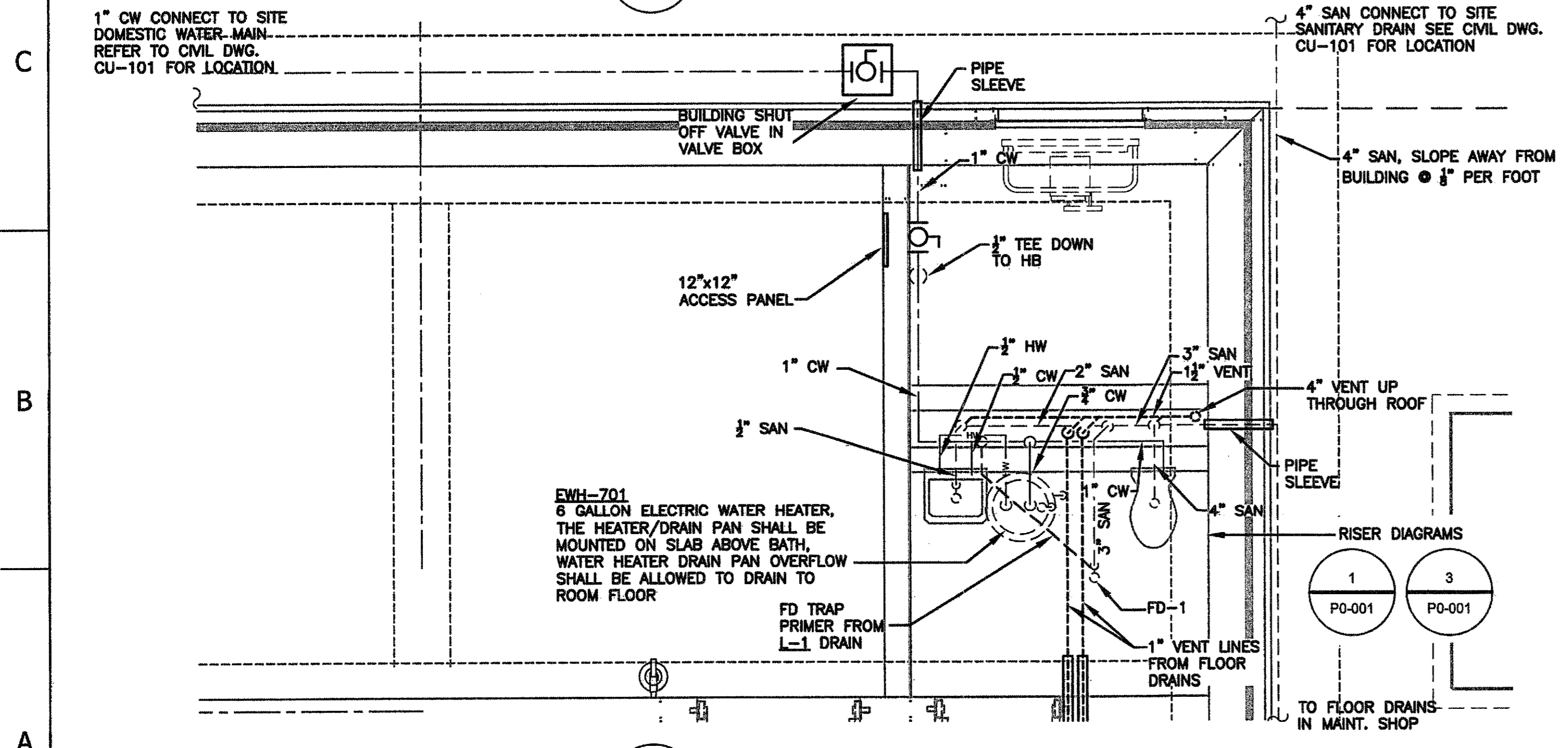
2 JET MIX STATION PLUMBING- ENLARGED BATH PLAN P7-101 SCALE: 3/8"=1'-0" FIN. FLR. EL. 839'-6"
