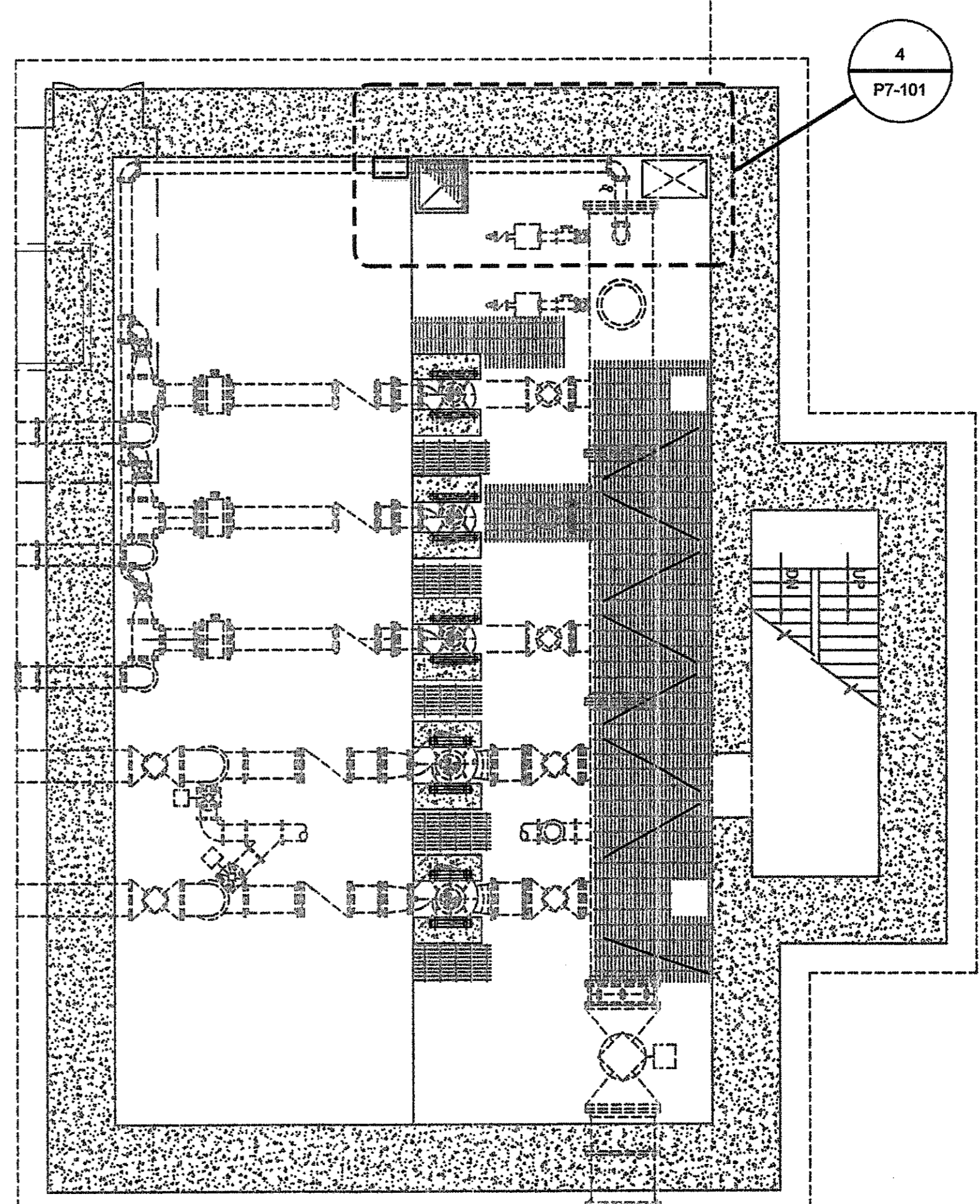
3 JET MIX STATION PLUMBING- LOWER LEVEL P7-101 SCALE: 3/8"=1'-0" FIN. FLR. EL. 795'-9"
