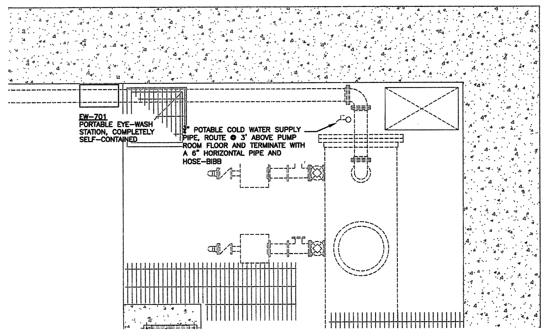
4 JET MIX STATION PLUMBING- ENLARGED LOWER LEVEL EYE-WASH P7-101 SCALE: 3/8"=1'-0" FIN. FLR. EL. 795'-9"
