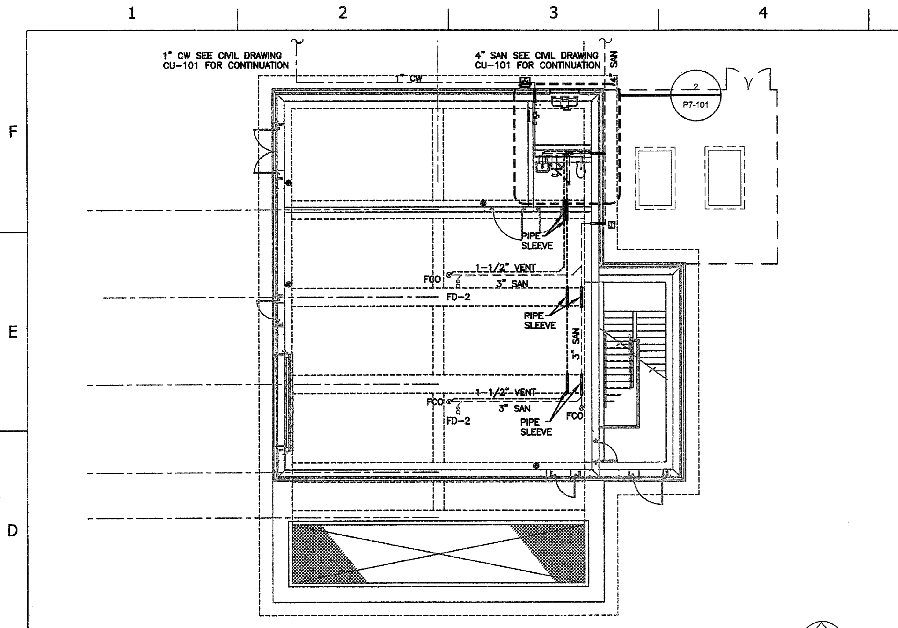
1 JET MIX STATION UPPER LEVEL PLUMBING PLAN P7-101 SCALE: 1/8"=1'-0" FIN. FLR. EL. 839'-6"
