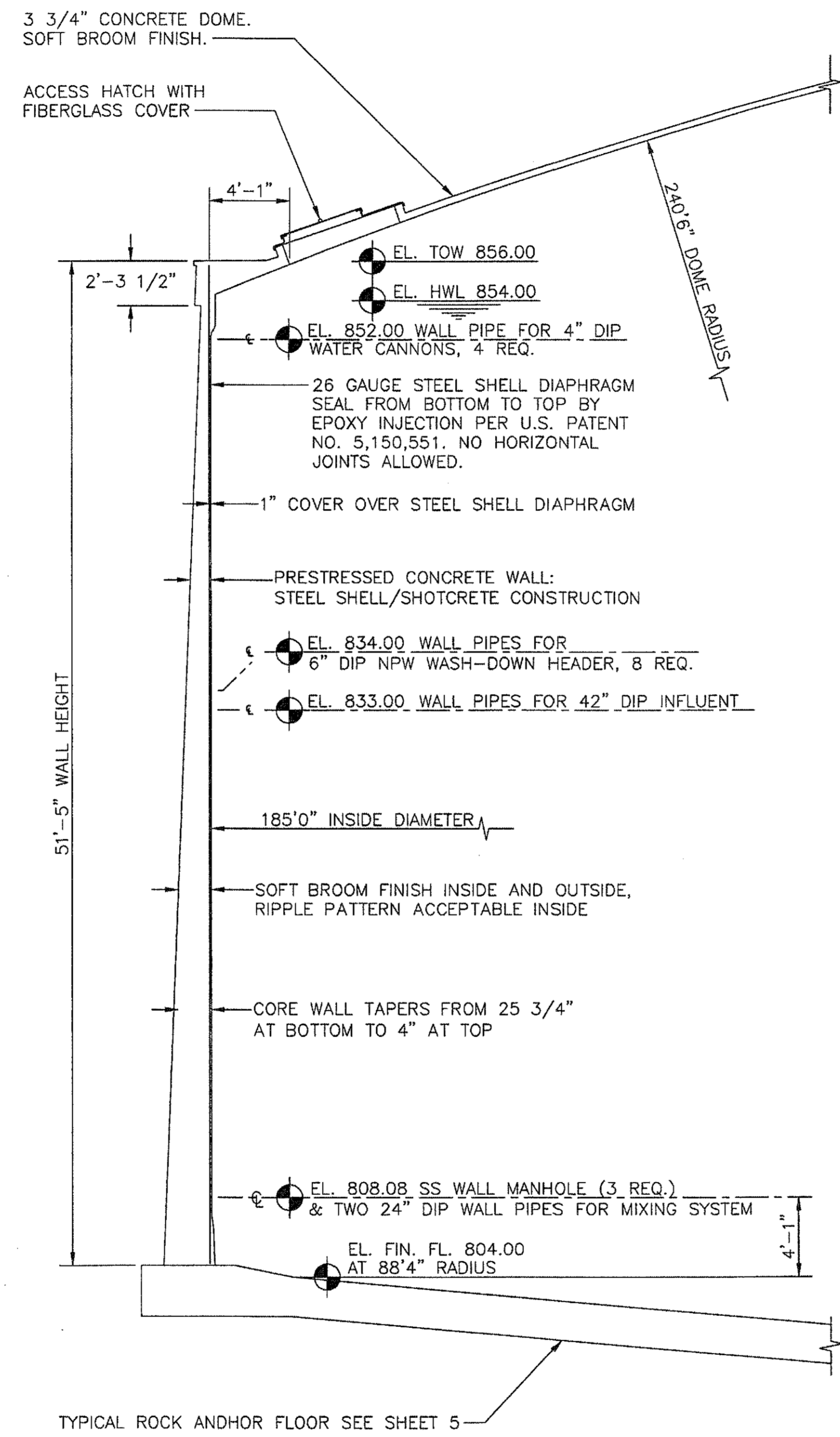
TYPICAL WALL DETAIL
