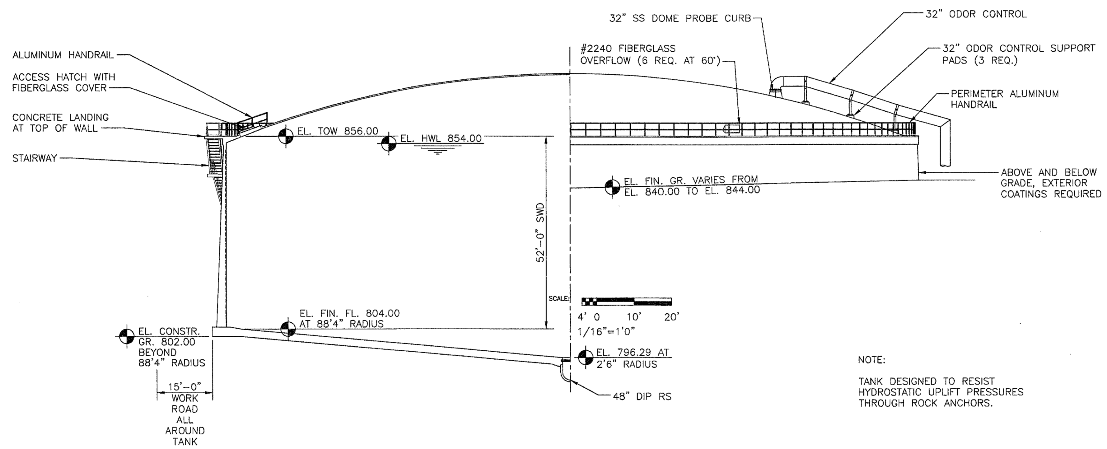
SECTION-ELEVATION
