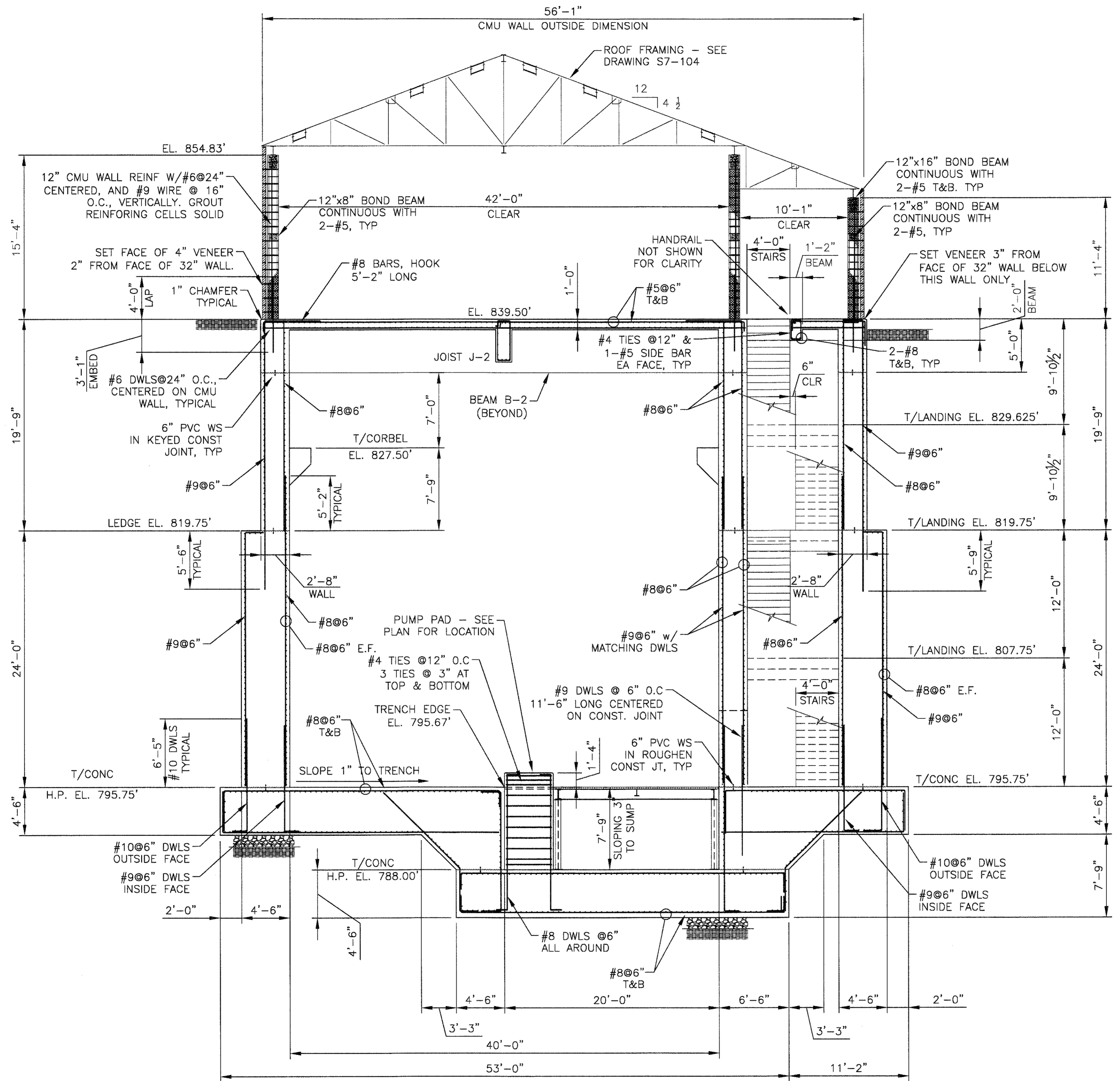
D SECTION S7-304 SCALE: 3/16" = 1'-0"
