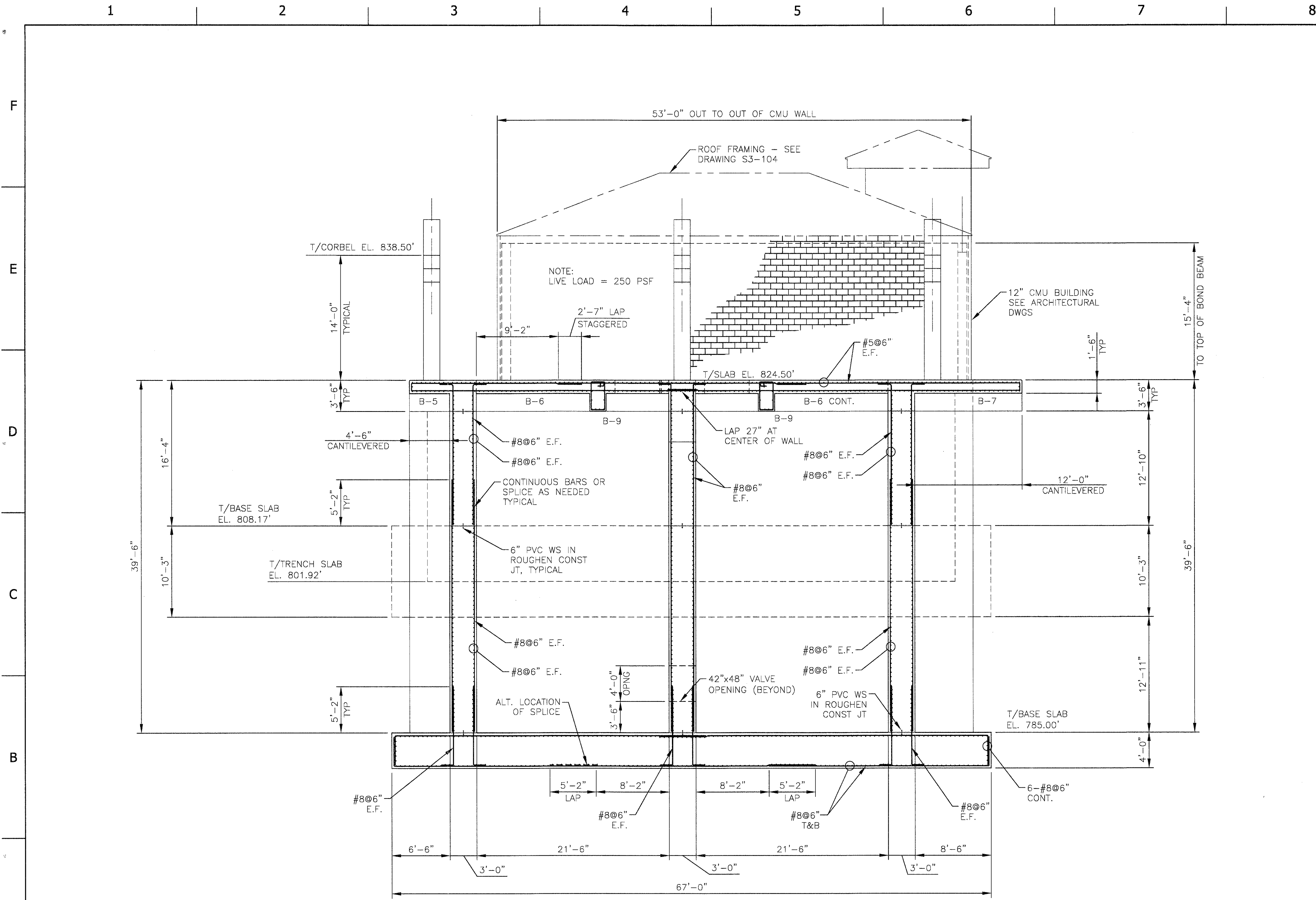
A SECTION S3-301 SCALE: 3/16" = 1'-0"
