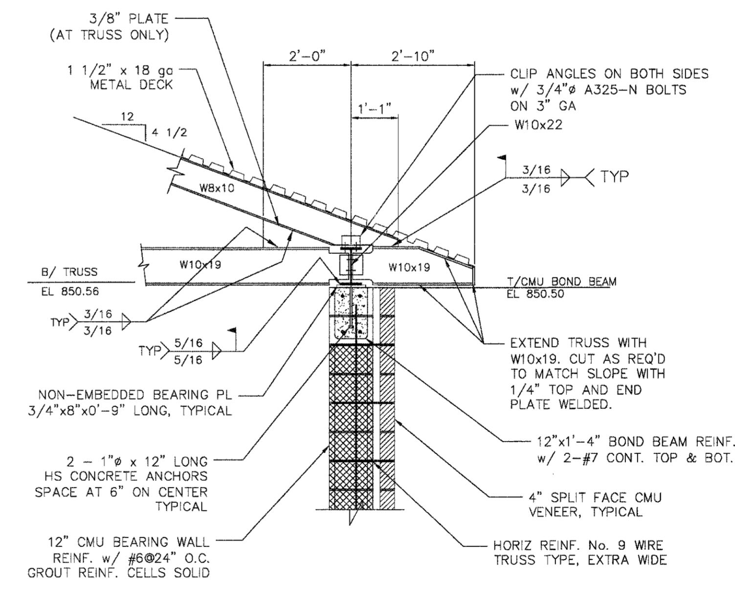
2 DETAIL S3-105 SCALE: NOT TO SCALE
