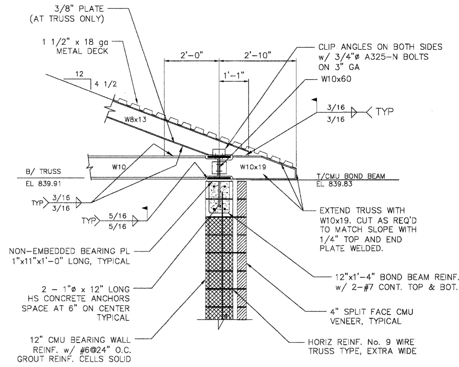
1 DETAIL S3-105 SCALE: NOT TO SCALE
