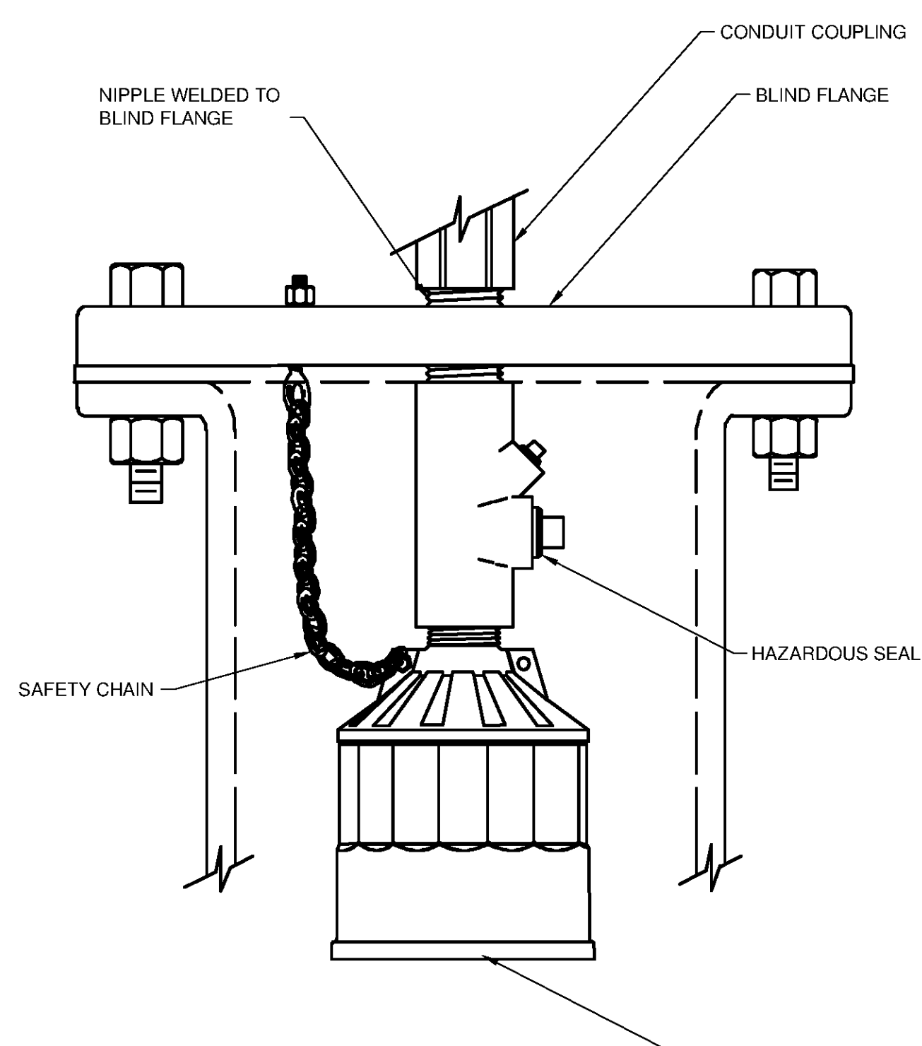
ULTRASONIC TRANSDUCER MOUNTING DETAIL
