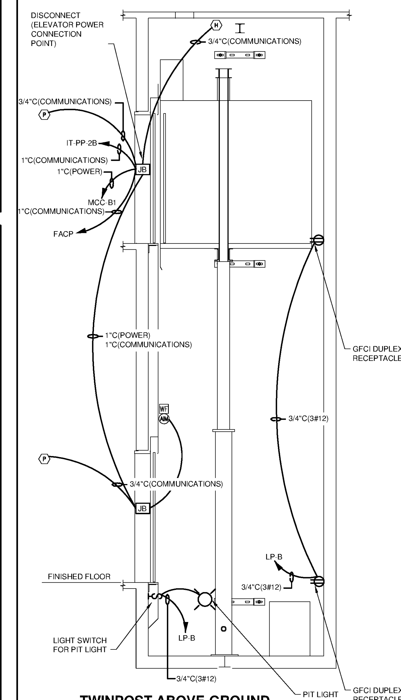
TWINPOST ABOVE-GROUND 2-STAGE ELEVATOR DETAIL
