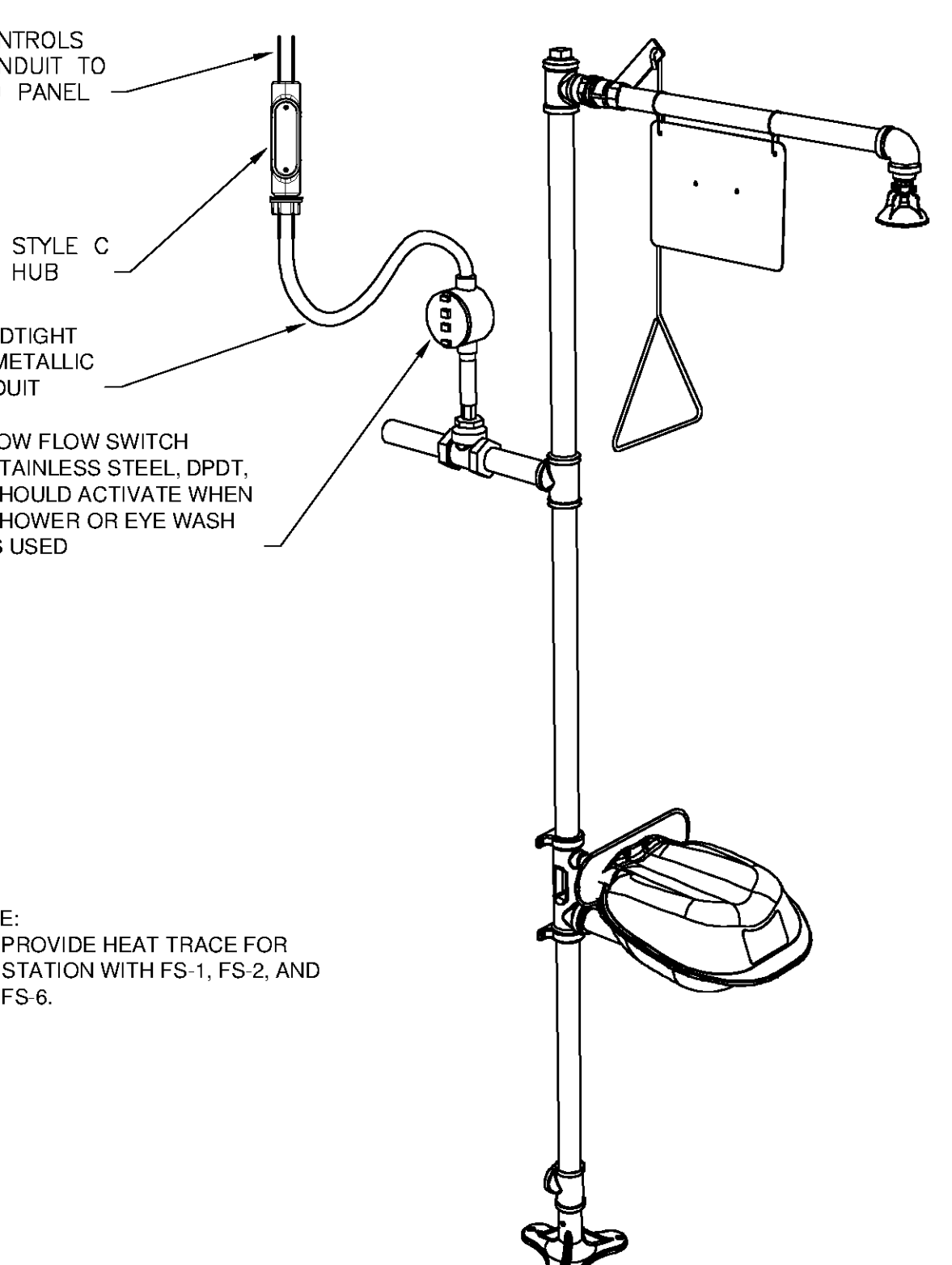
FLOW SWITCH EYE/SOWER WASH STATION DETAIL
