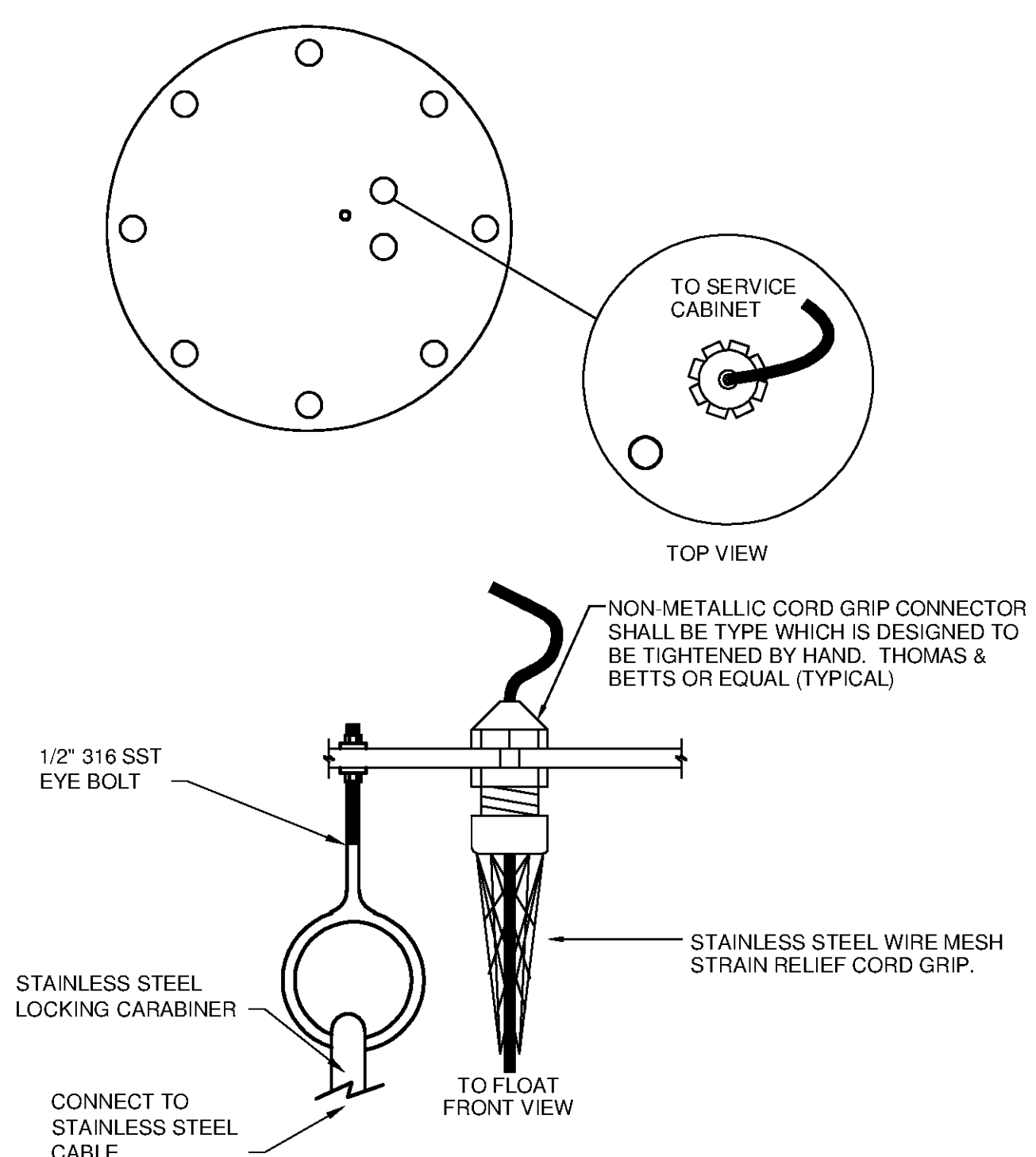
ELEVATED TANK CABLE SUPPORT DETAIL
