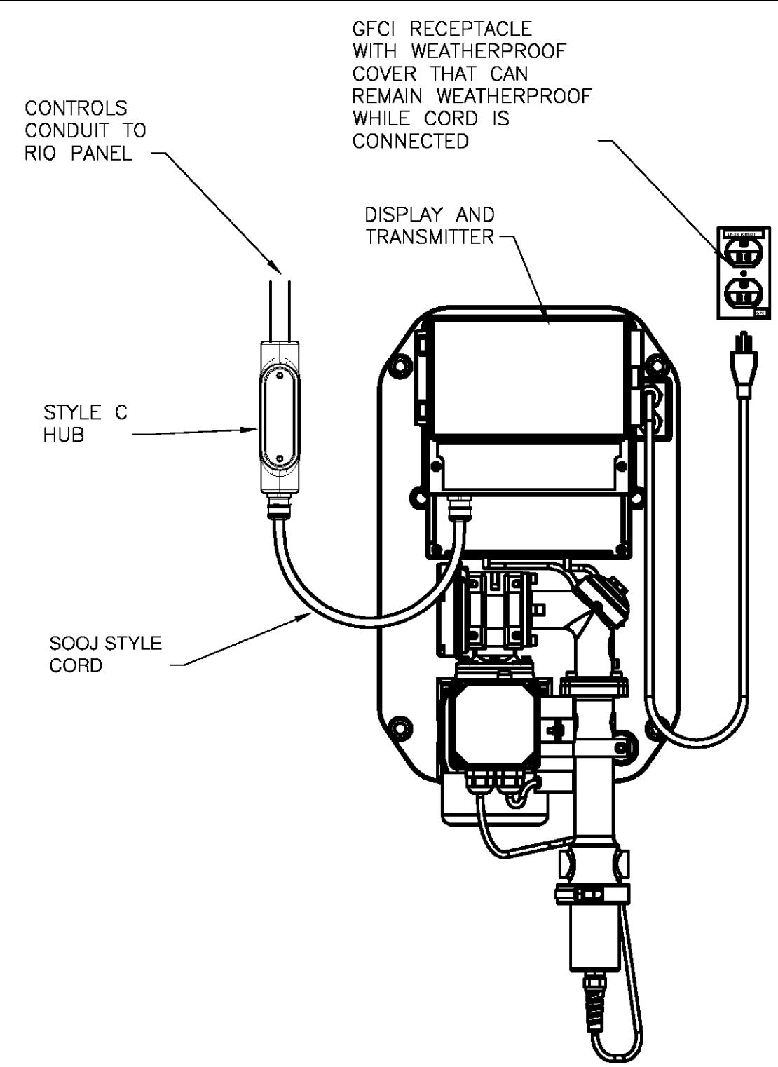
STREAMING CURRENT PROBE MOUNTING DETAIL (IN-LINE TYPE)
