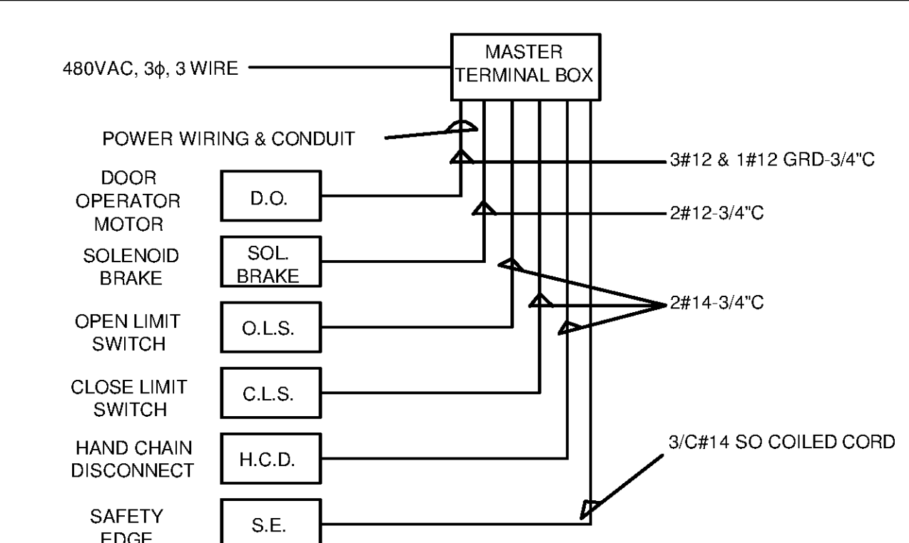
OVERHEAD DOOR RISER DIAGRAM
