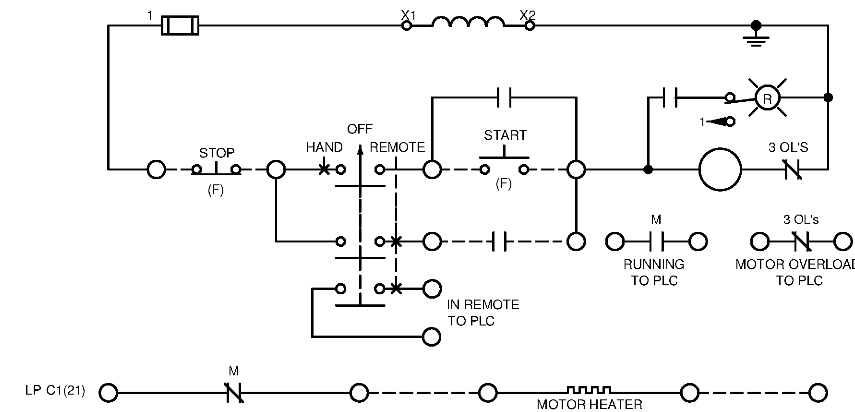
RADIATOR FAN WIRING DIAGRAM TYP. GENSETS 1-4 SCALE: N/A
