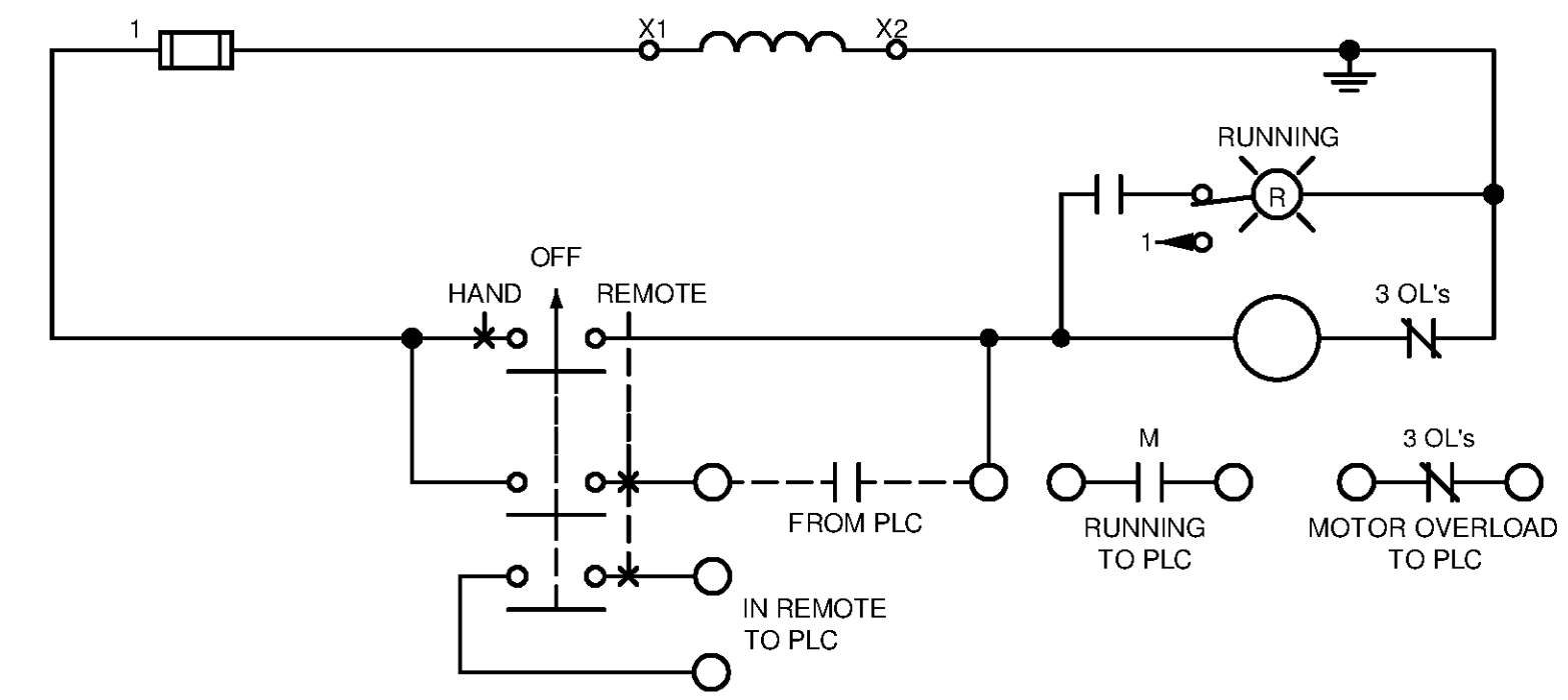
COOLING WATER PUMP WIRING DIAGRAM TYP. GENSETS 1-4 SCALE: N/A
