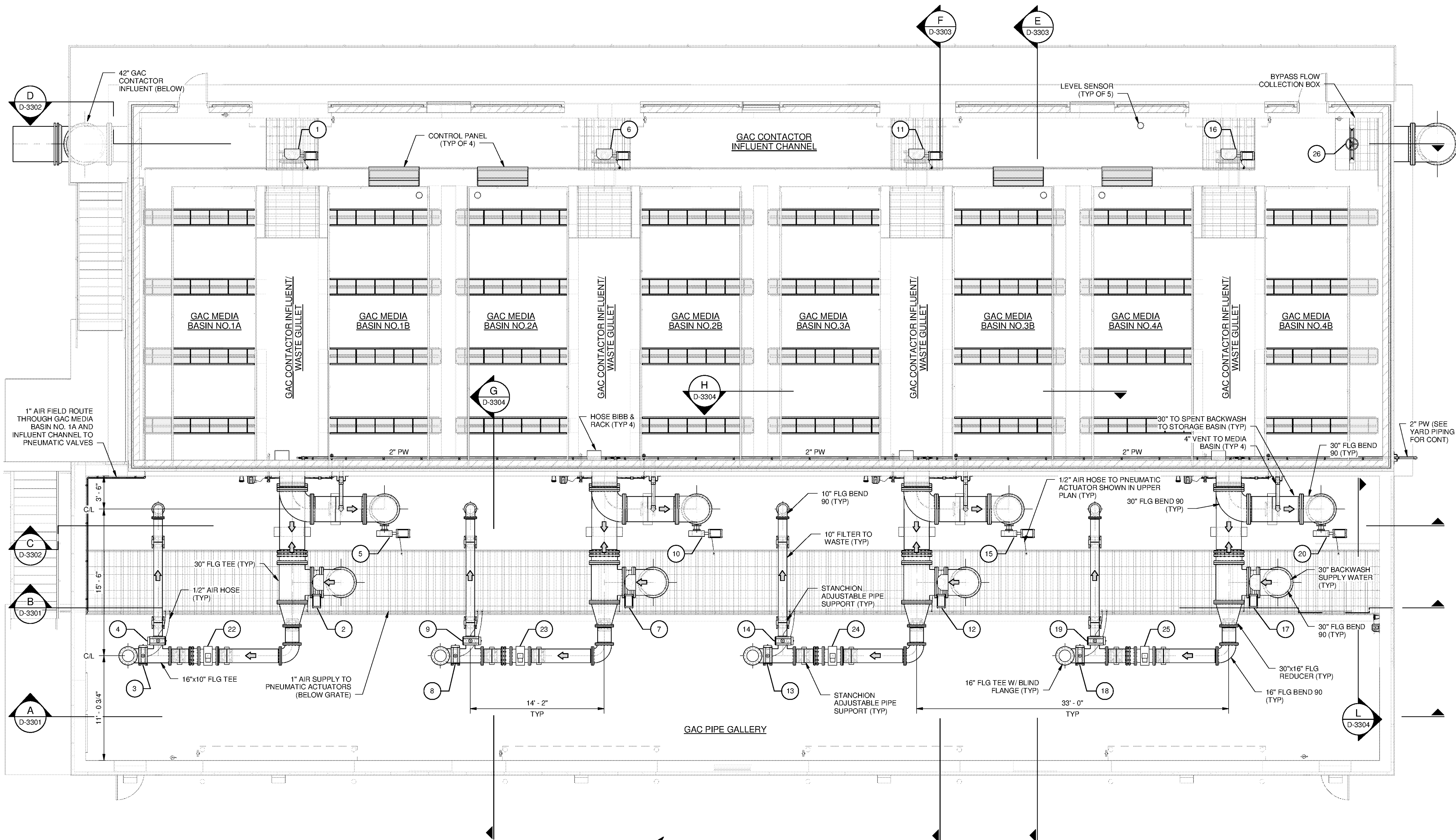
PLAN @ EL 632'-6" SCALE: 3/16" = 1'-0"
