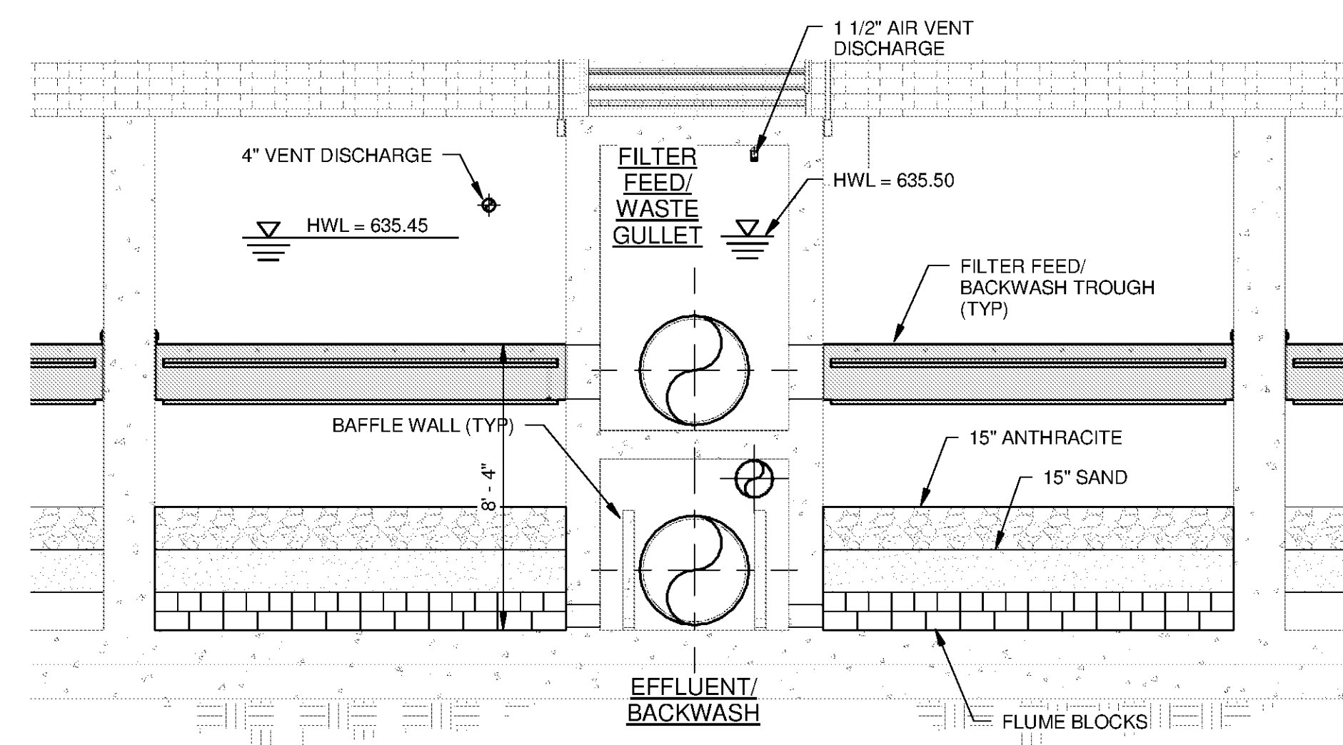
H SECTION D-2106 SCALE: 1/4" = 1'-0"
