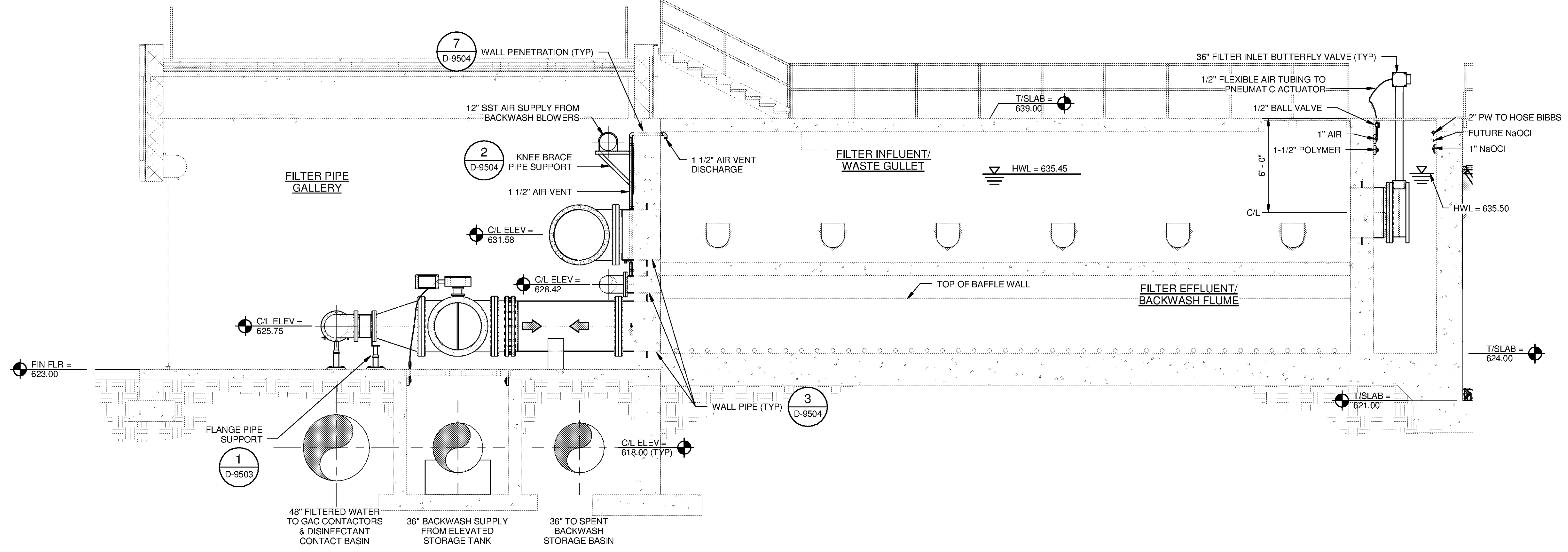
F SECTION D-2106 SCALE: 1/4" = 1'-0"
