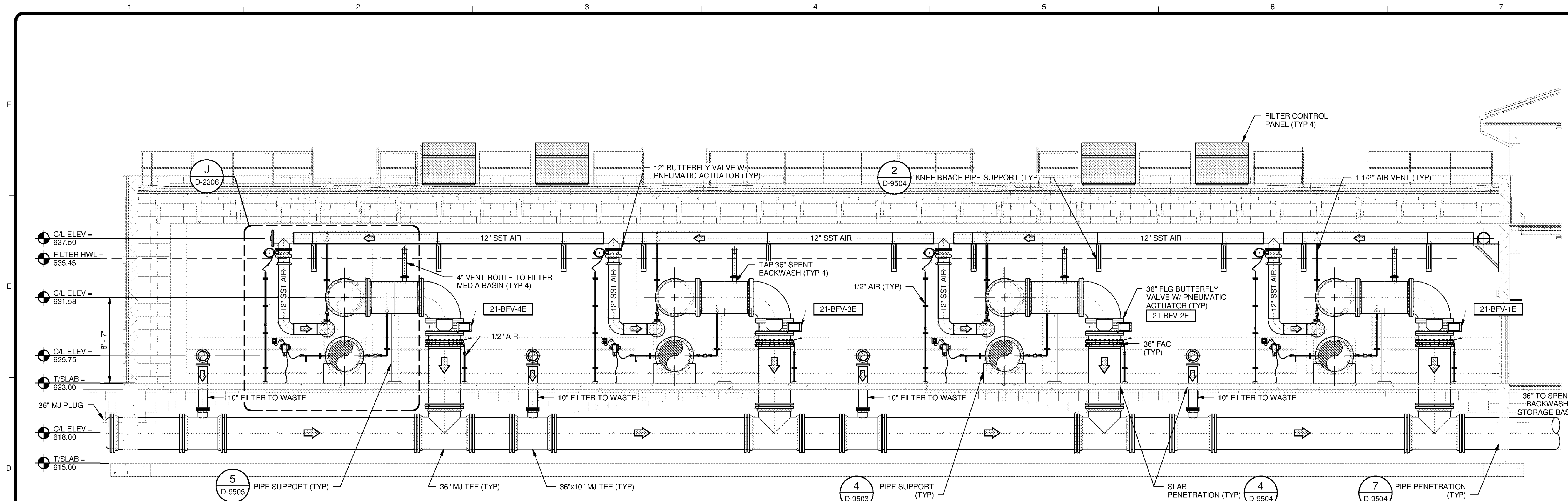
C SECTION D-2106 SCALE: 3/16" = 1'-0"
