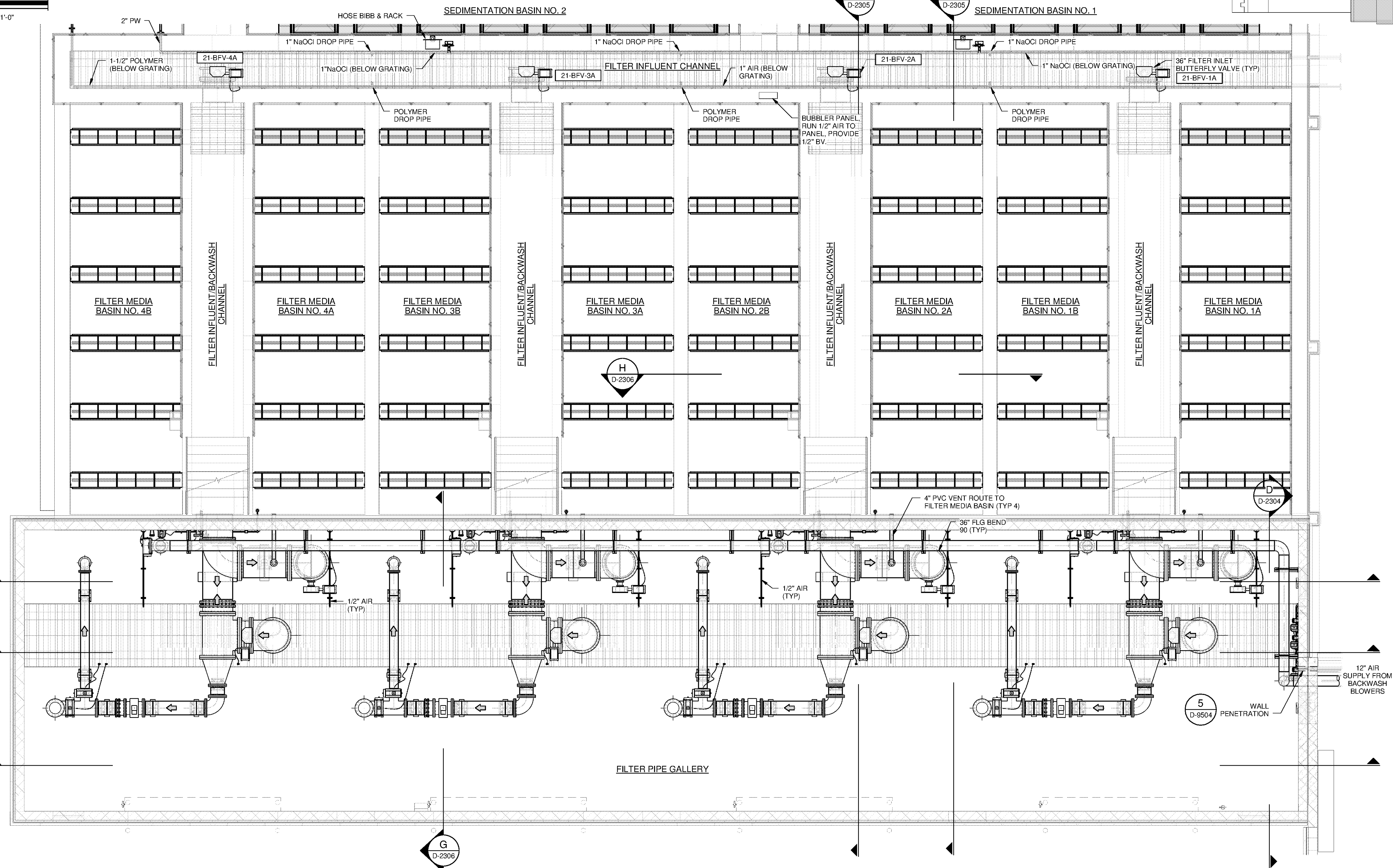
PLAN SCALE: 3/16" = 1'-0"
