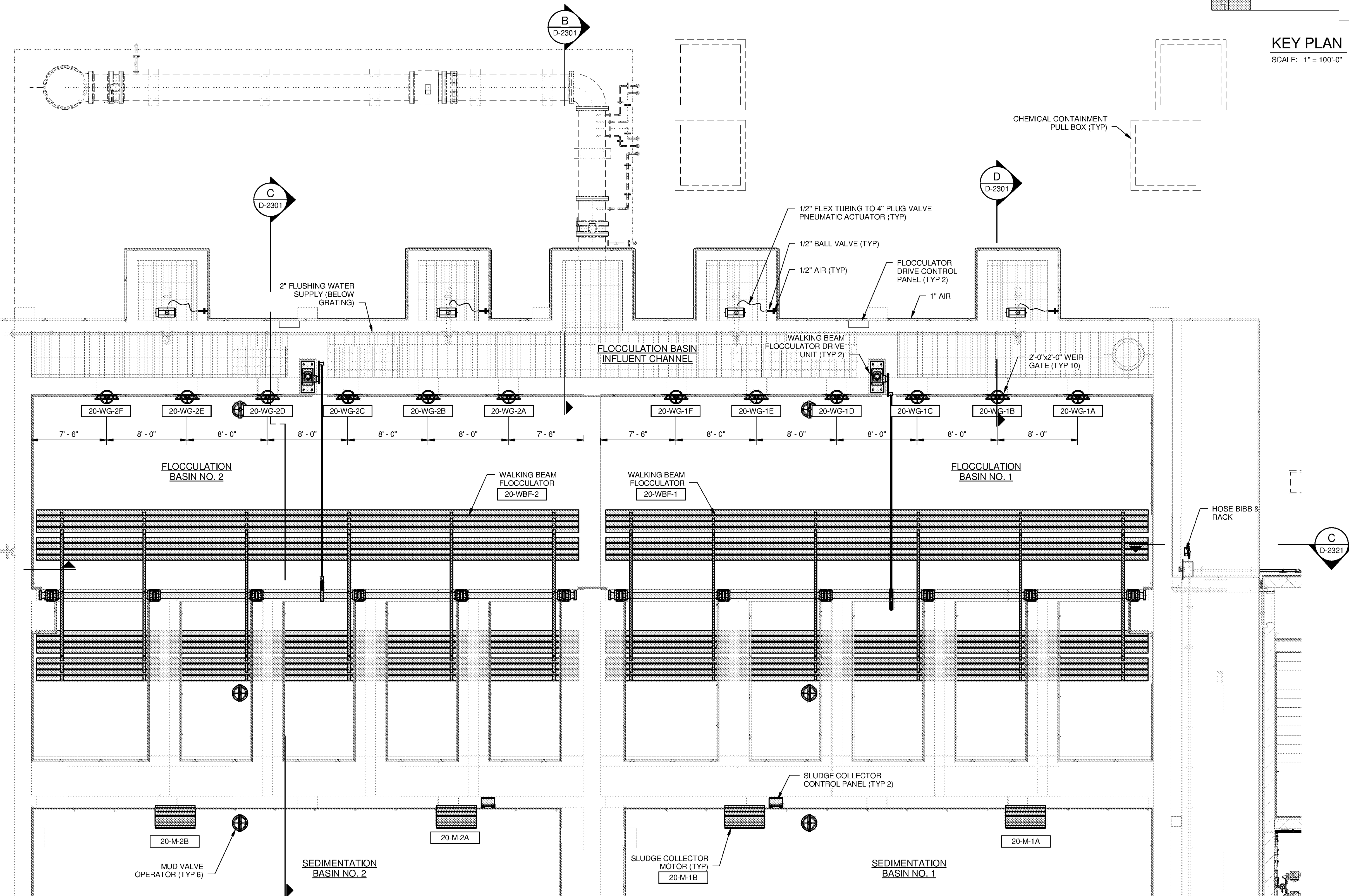
PLAN SCALE: 3/16" = 1'-0"
