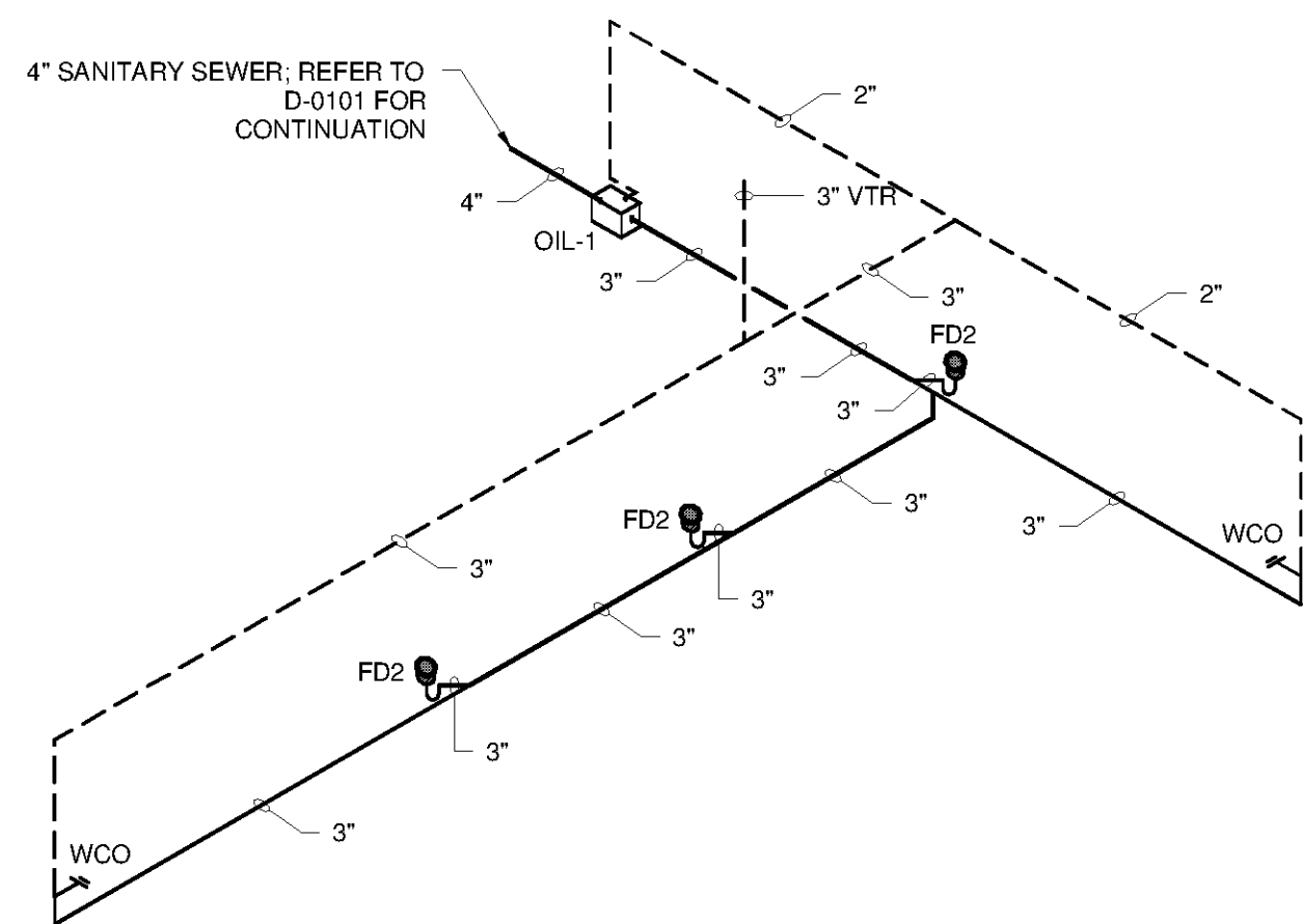
2 GENERATOR BUILDING SANITARY SEWER RISER DIAGRAM SCALE: N.T.S.
