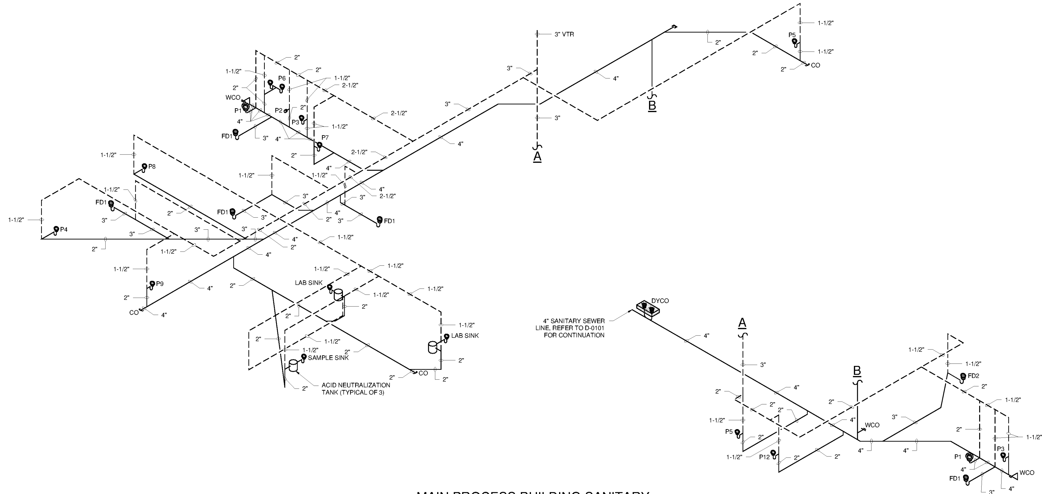
1 MAIN PROCESS BUILDING SANITARY SEWER RISER DIAGRAM SCALE: N.T.S.
