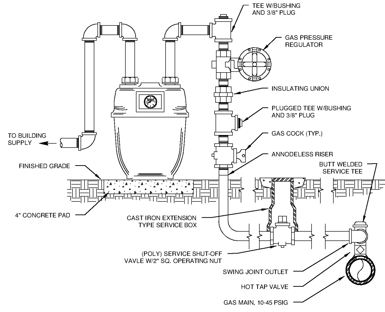
1 GAS SERVICE CONNECTION DETAIL SCALE: N.T.S.
