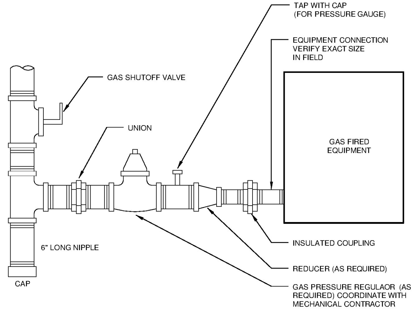
2 GAS FIRED EQUIPMENT CONNECTION SCALE: N.T.S.
