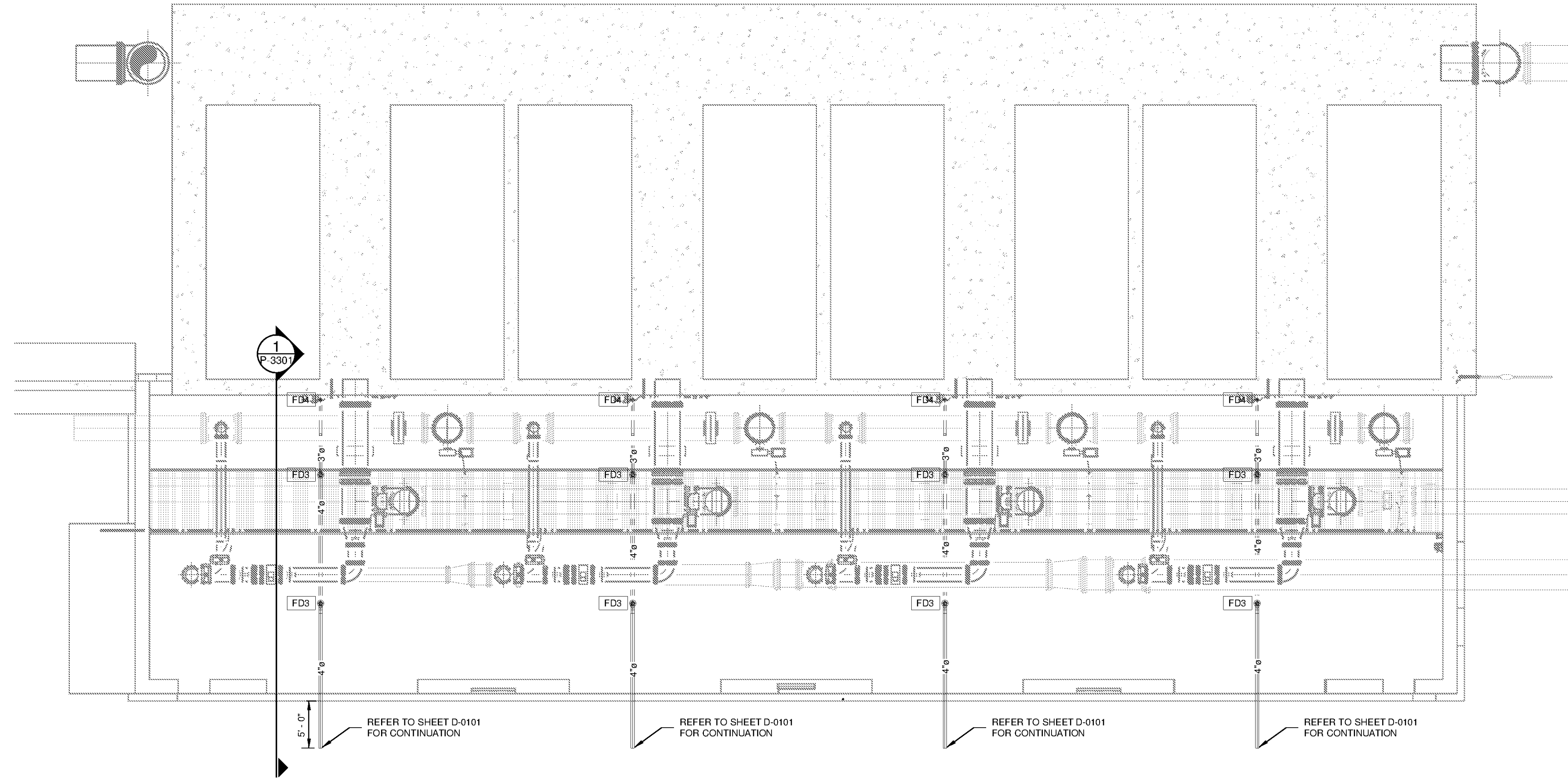
GAC/BAC FILTRATION BUILDING PLUMBING FLOOR PLAN SCALE: 1/8" = 1'-0"
