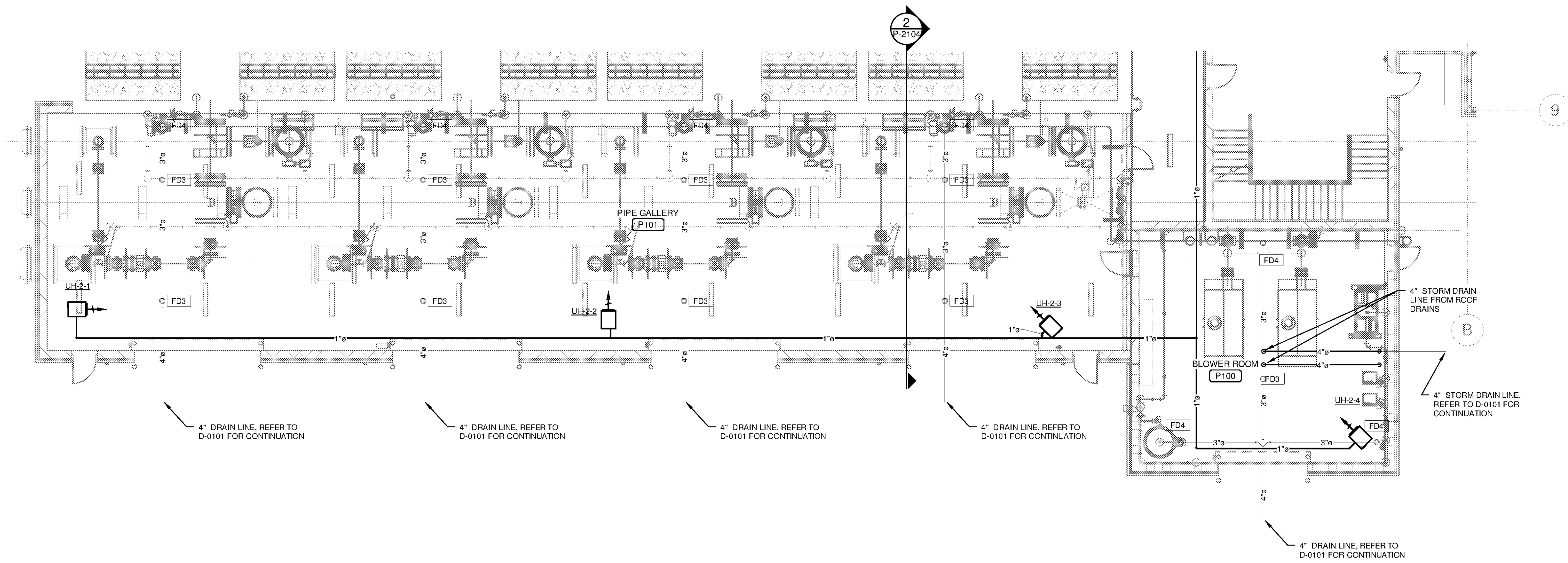
PIPE GALLERY PLUMBING PLAN SCALE: 1/8" = 1'-0"
