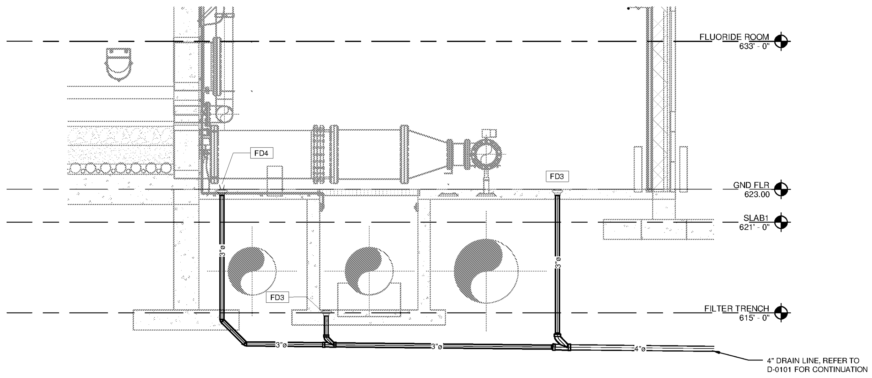
PIPE GALLERY SECTION SCALE: 1/4" = 1'-0"
