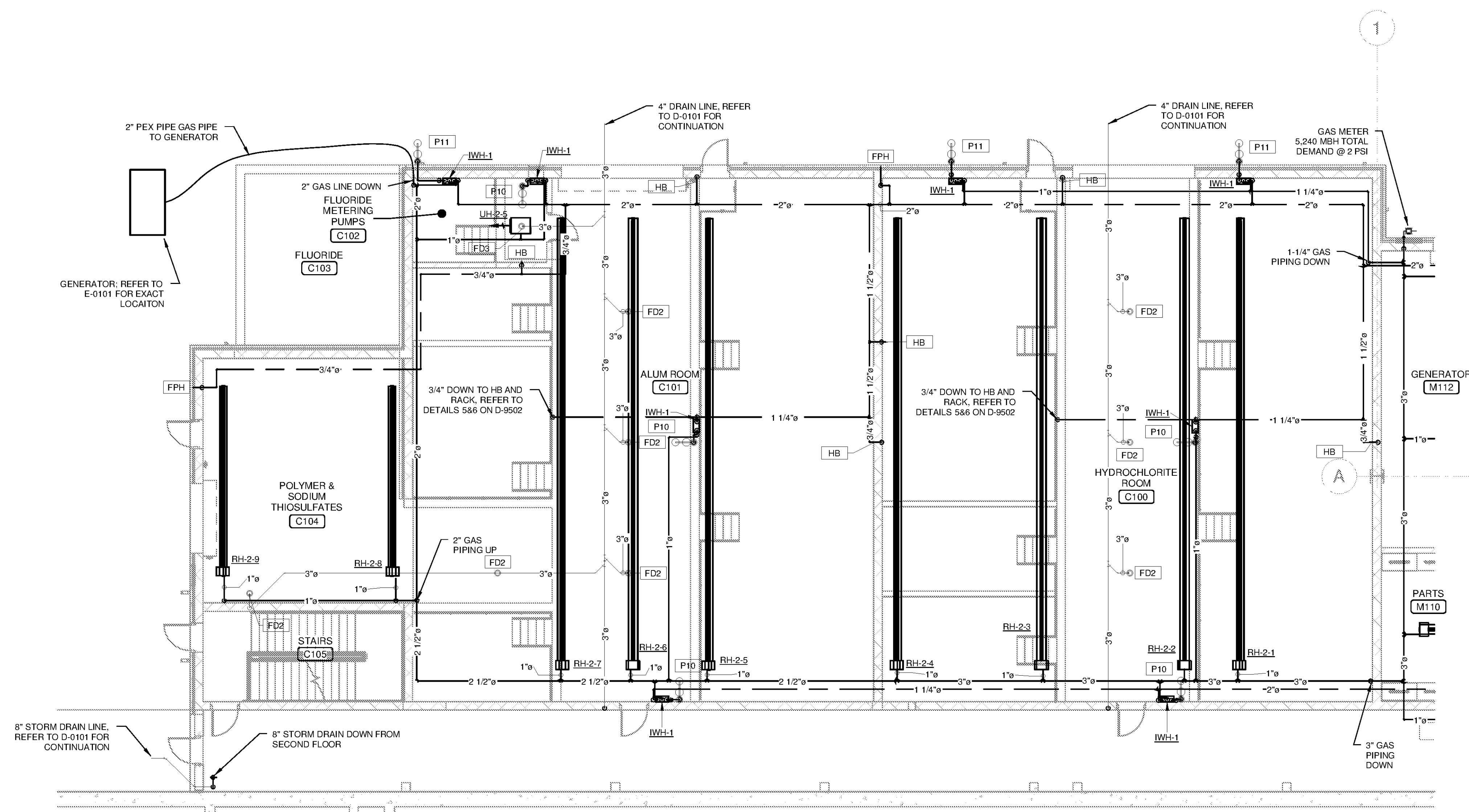
CHEMICAL FEED PLUMBING PLAN SCALE: 1/8" = 1'-0"
