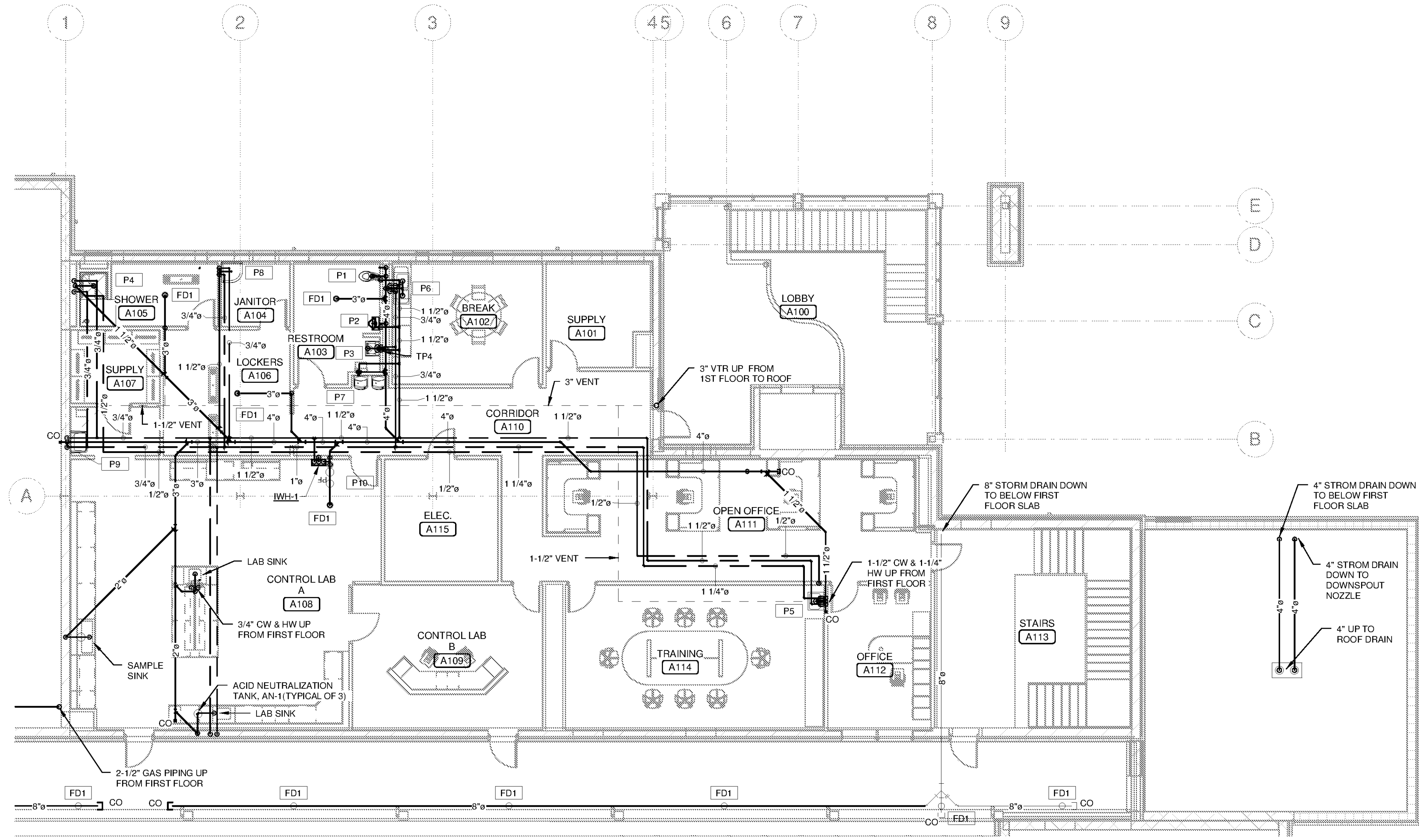
OPERATIONS SECOND FLOOR PLUMBING PLAN
