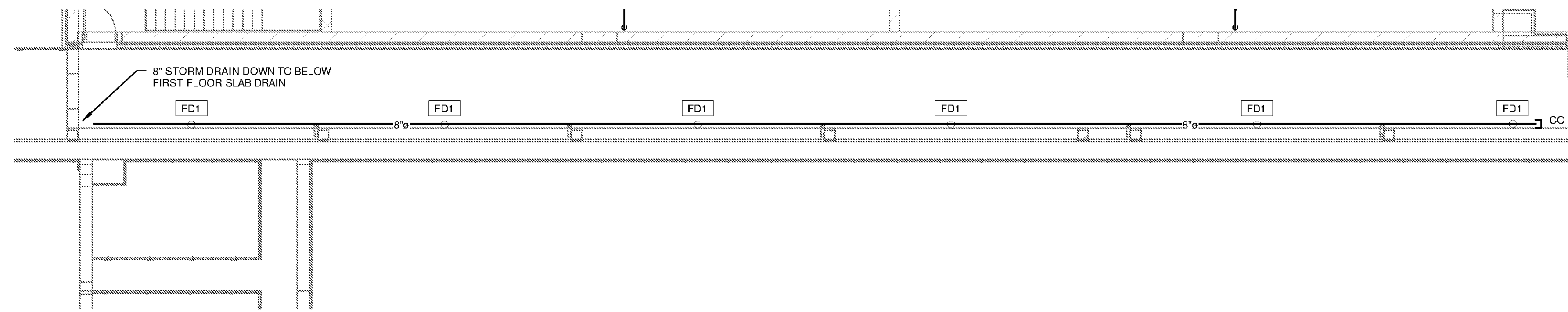
CHEMICAL FEED SECOND FLOOR PLUMBING PLAN
