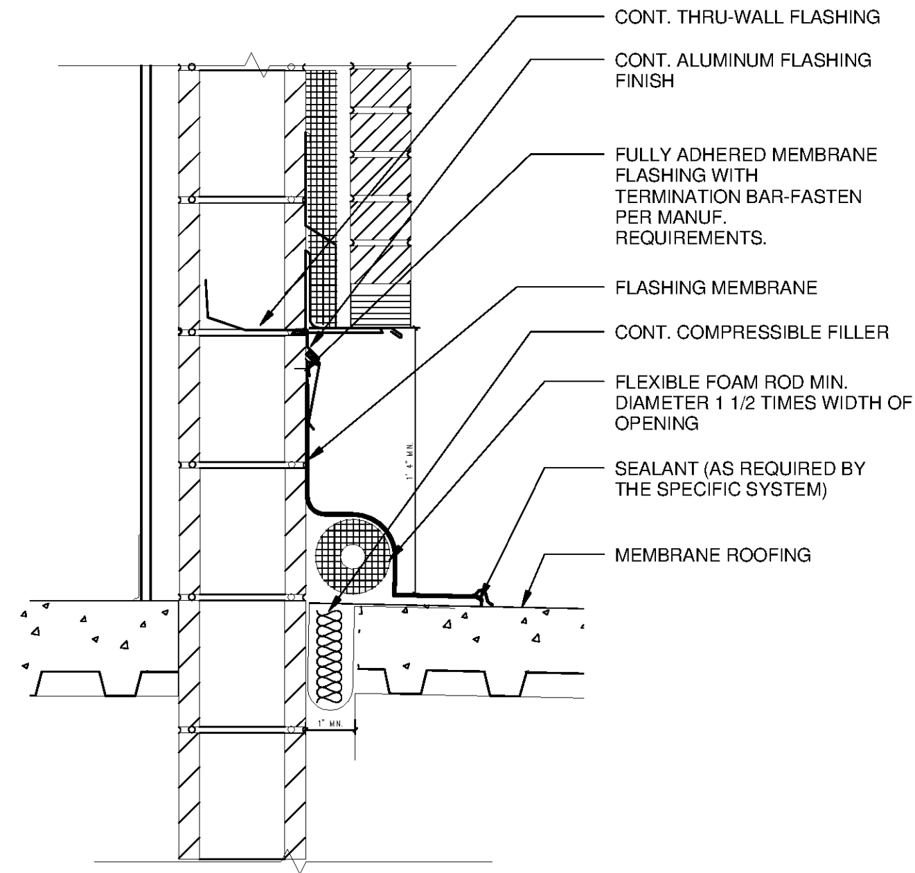
14 EXPANSION JOINT AT DECK SCALE: 1 1/2" = 1'-0"
