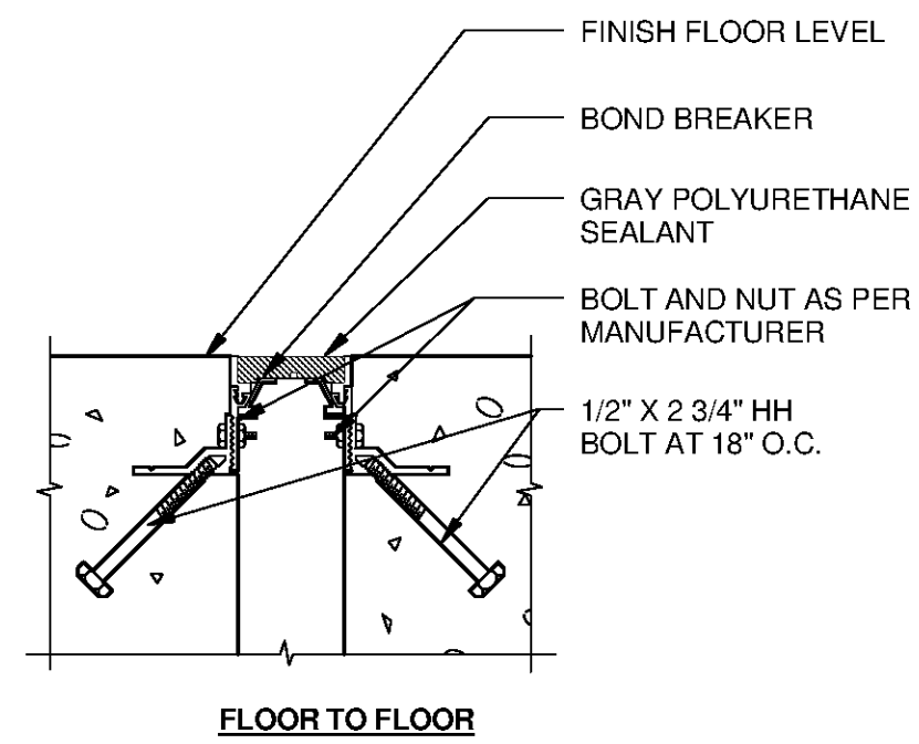
15 EXPANSION JOINT DETAIL AT BASIN SCALE: 3" = 1'-0"
