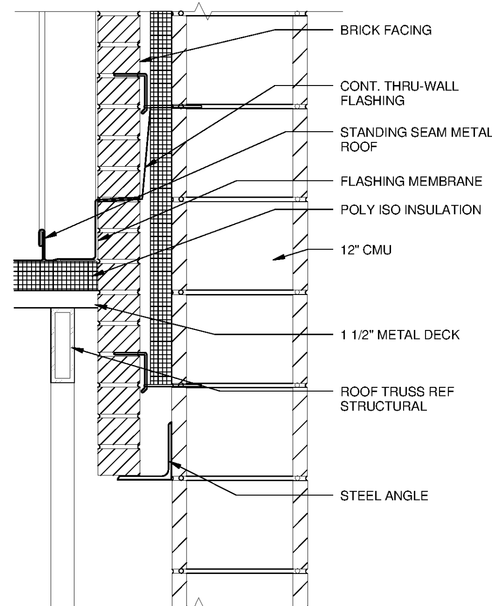
13 RAKE AT UPPER WALL SCALE: 1 1/2" = 1'-0"
