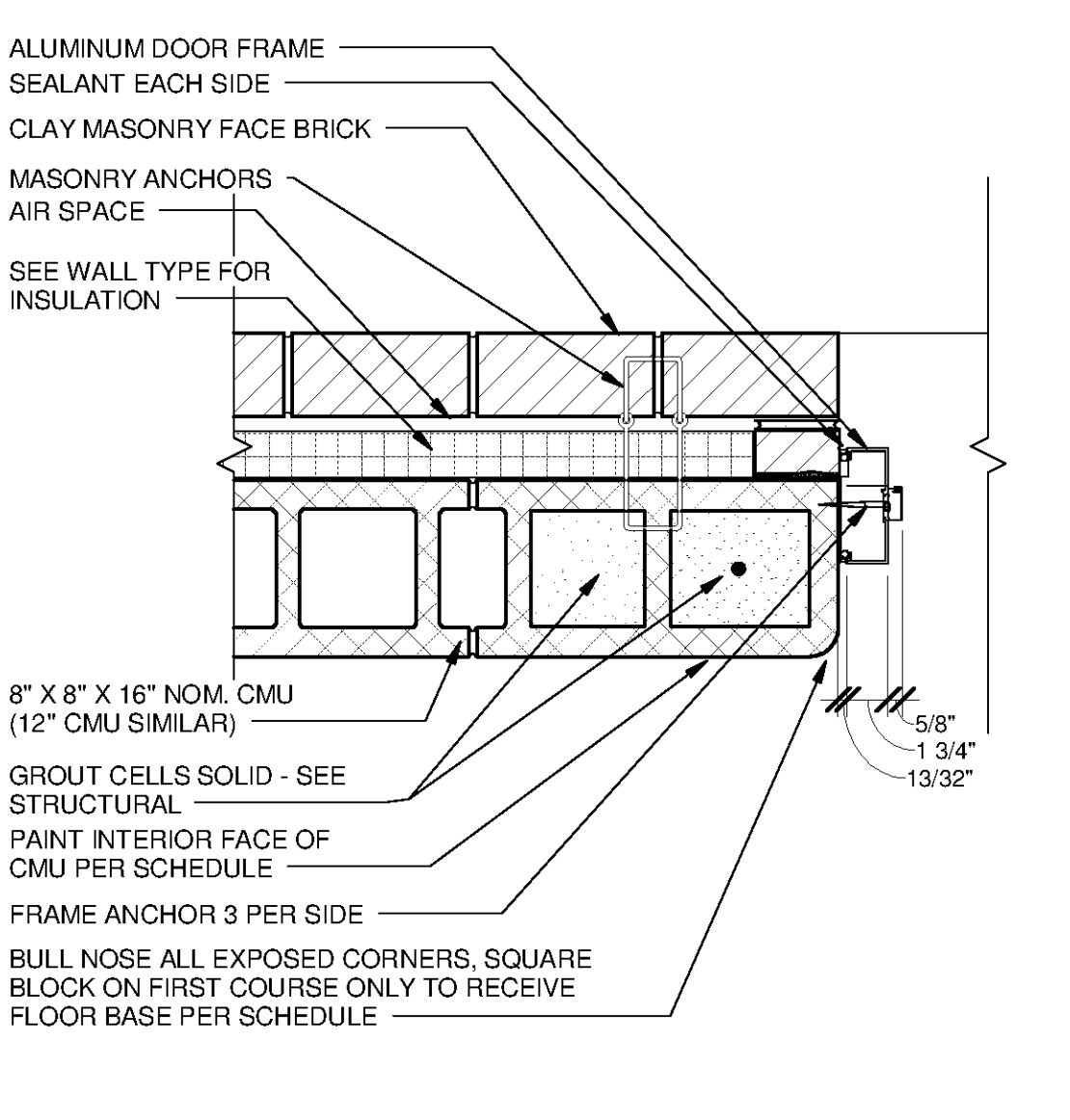
2 DOOR JAMB TYPE A SCALE: 1 1/2" = 1'-0"
