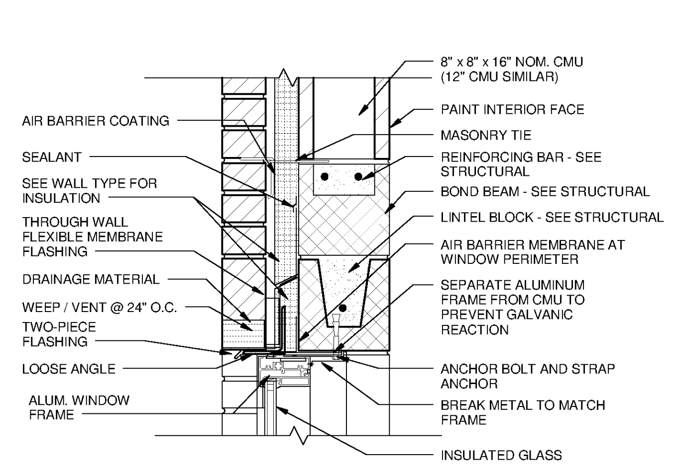
7 WINDOW HEAD TYPE WH-A SCALE: 1 1/2" = 1'-0"
