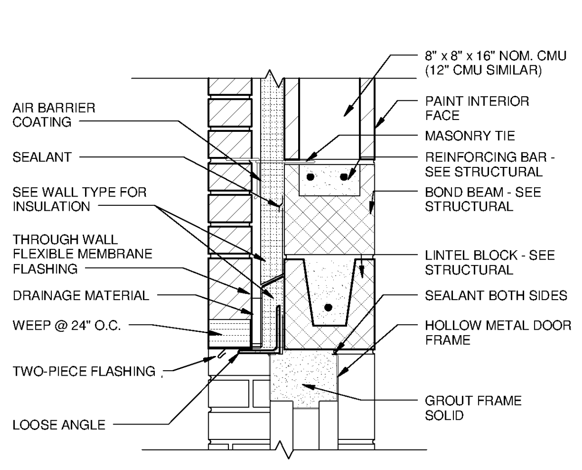
4 DOOR HEAD TYPE A.1 SCALE: 1 1/2" = 1'-0"
