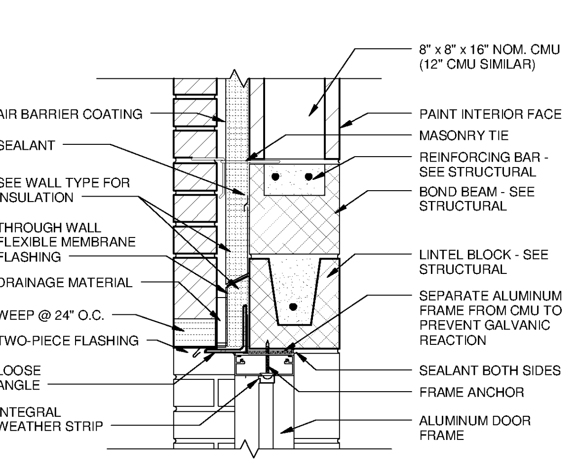
1 DOOR HEAD TYPE A SCALE: 1 1/2" = 1'-0"
