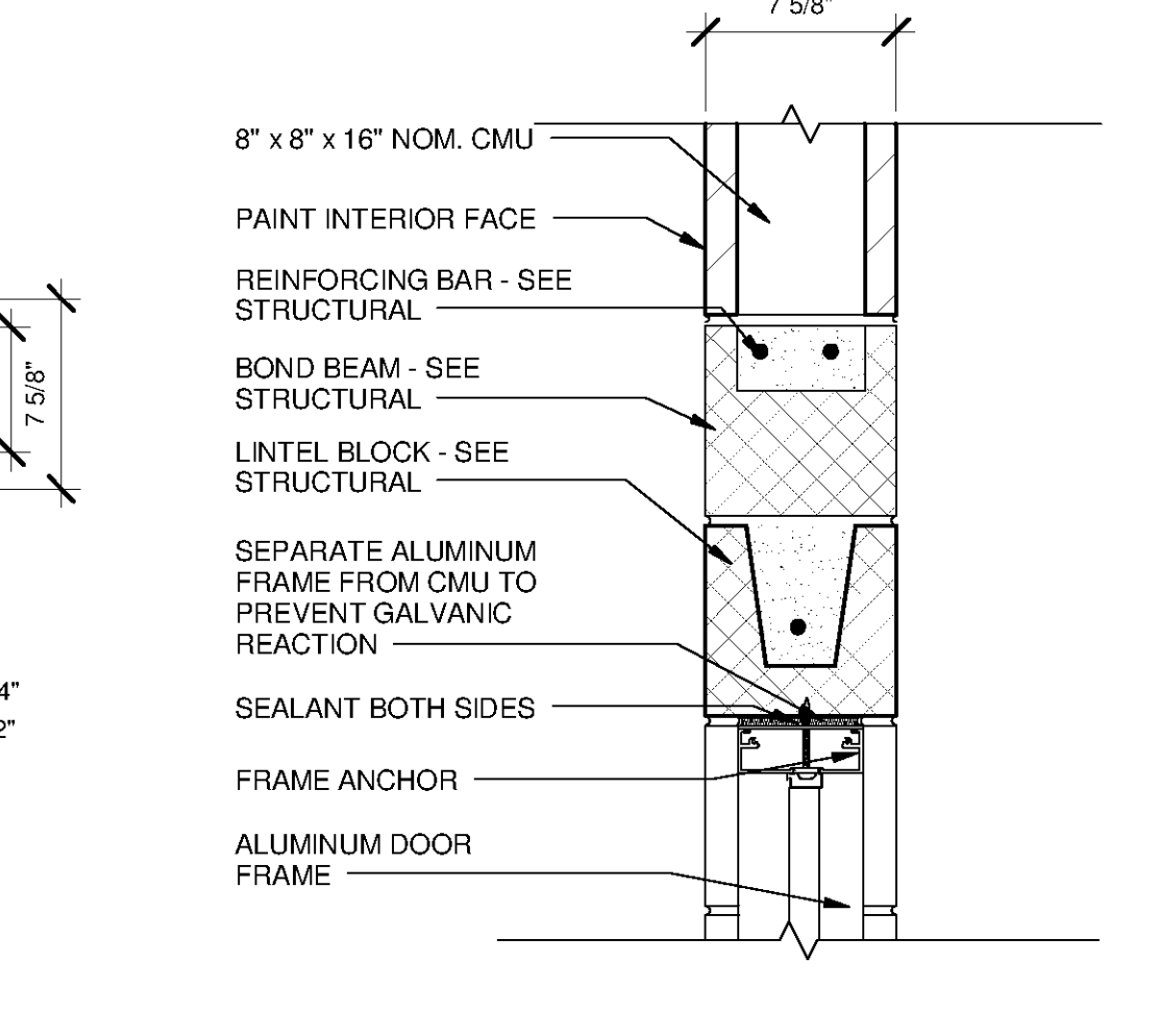
3 DOOR HEAD TYPE B SCALE: 1 1/2" = 1'-0"
