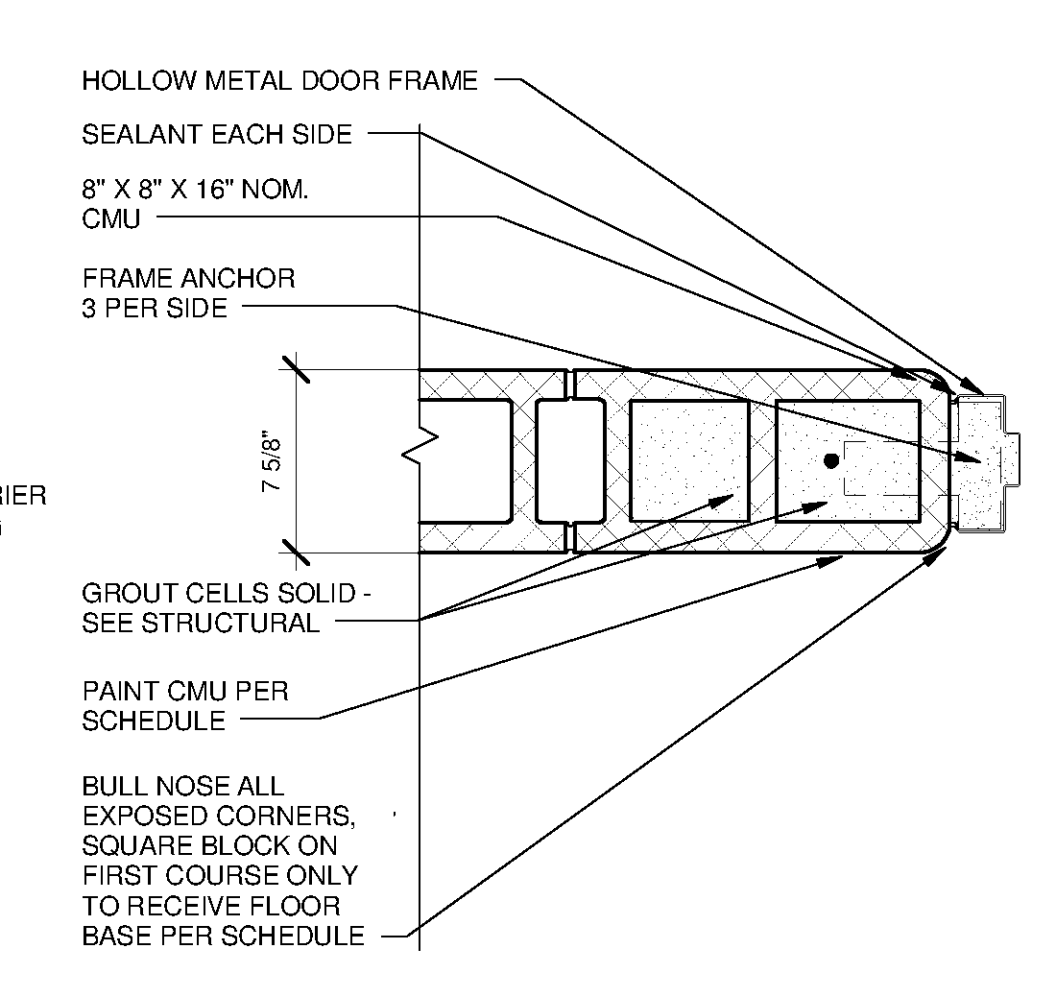
11 DOOR JAMB TYPE B.1 SCALE: 1 1/2" = 1'-0"
