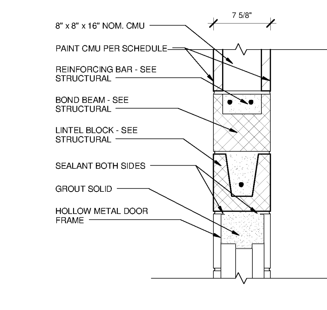
9 DOOR HEAD TYPE B.1 SCALE: 1 1/2" = 1'-0"
