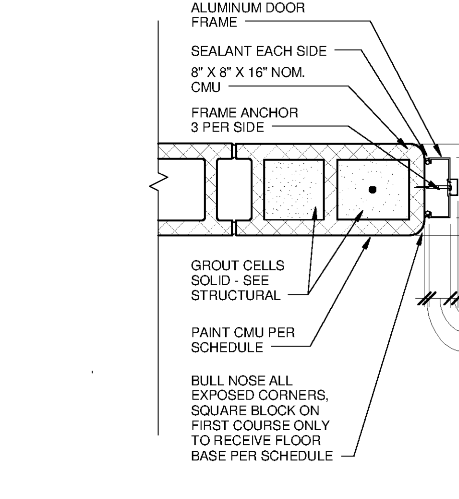
6 DOOR JAMB TYPE B SCALE: 1 1/2" = 1'-0"
