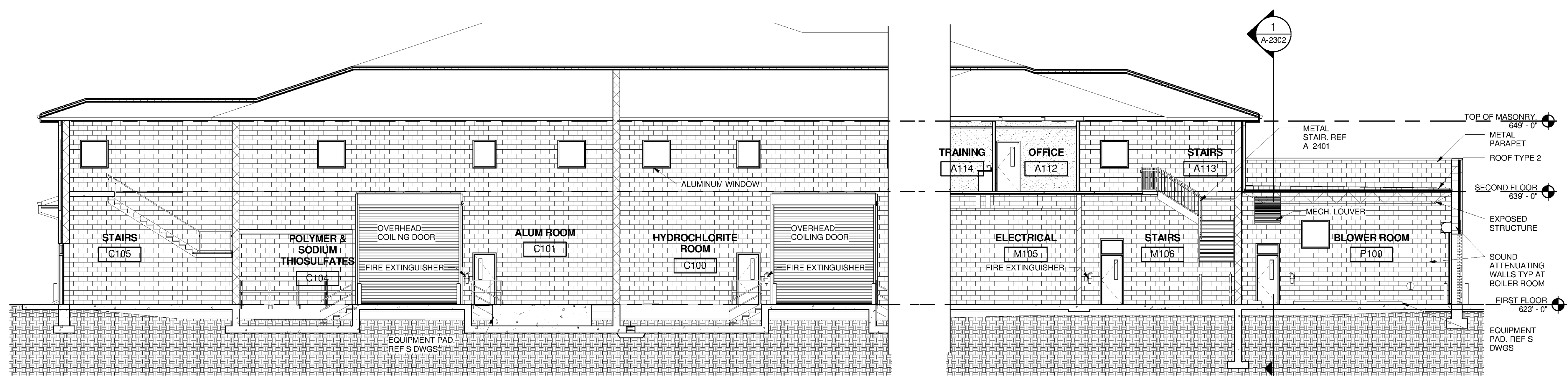
2 SECTION AT ALUM RM./ADMIN A-2102 SCALE: 1/8" = 1'-0"
