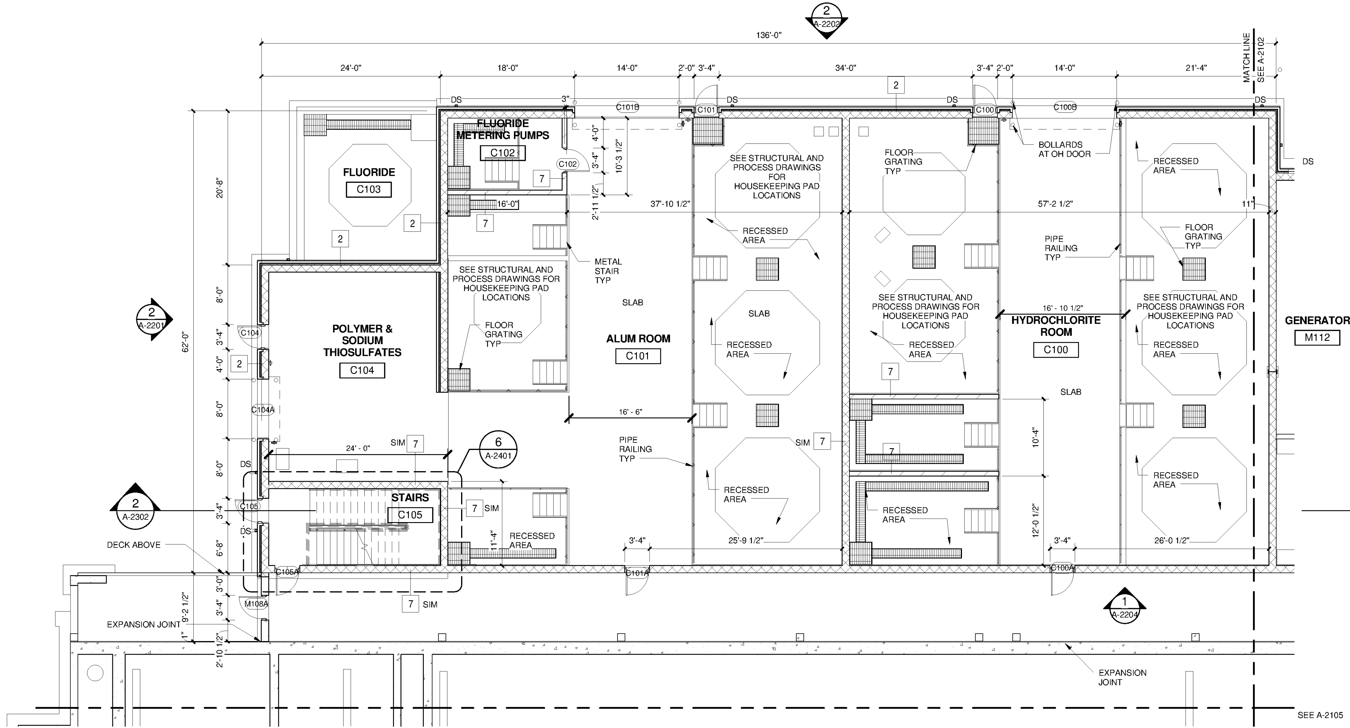
CHEM FEED FIRST FLOOR PLAN ELEV. 623 SCALE: 1/8" = 1'-0"
