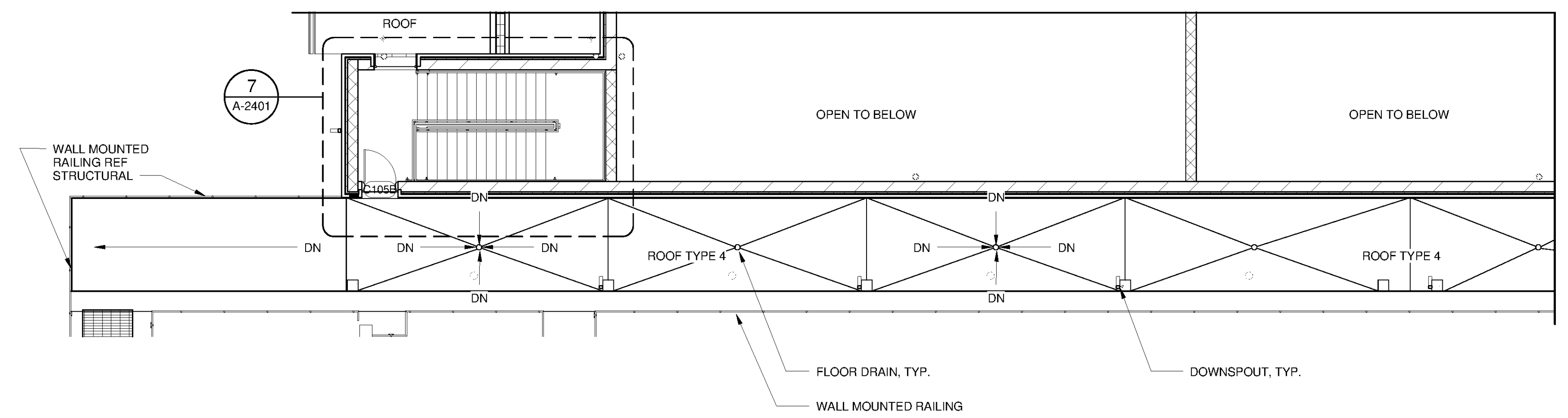
CHEM FEED 2ND FLOOR PLAN - ELEV. 639 SCALE: 1/8" = 1'-0"
