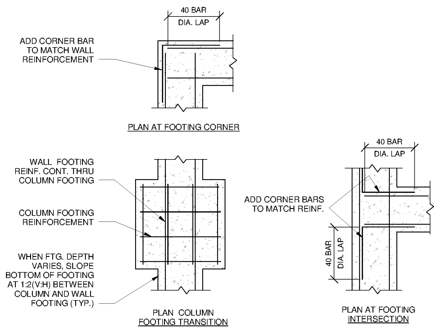
7 TYP. FOOTING INTERSECTIONS SCALE: 3/4" = 1'-0"
