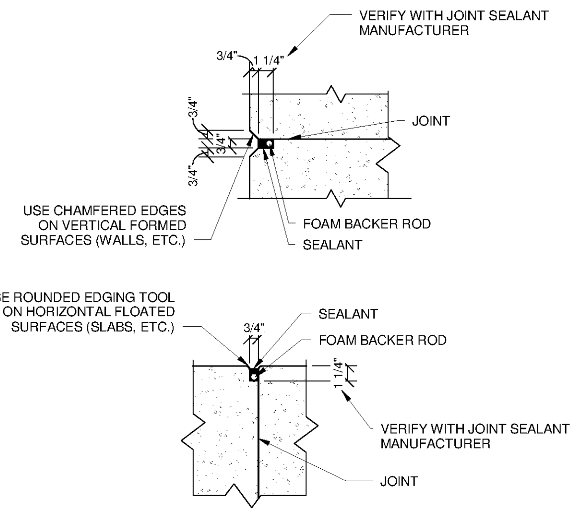
1 CONTROL JOINT SEALANT SCALE: 1 1/2" = 1'-0"
