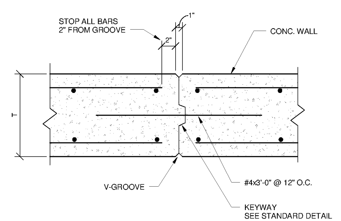
4 CONSTRUCTION JOINT @ BLDG. WALLS SCALE: 1 1/2" = 1'-0" NOTE: 1. MAX. CONST. JT. SPACING = 60'-0" O.C. 2. A CONSTRUCTION JT. SHALL BE LOCATED WITHIN 15'-0" OF A WALL CORNER. 3. ADJACENT WALL POURS SHALL BE DELAYED 2 DAYS MIN. TO ALLOW CURING OF PREVIOUS POUR.
