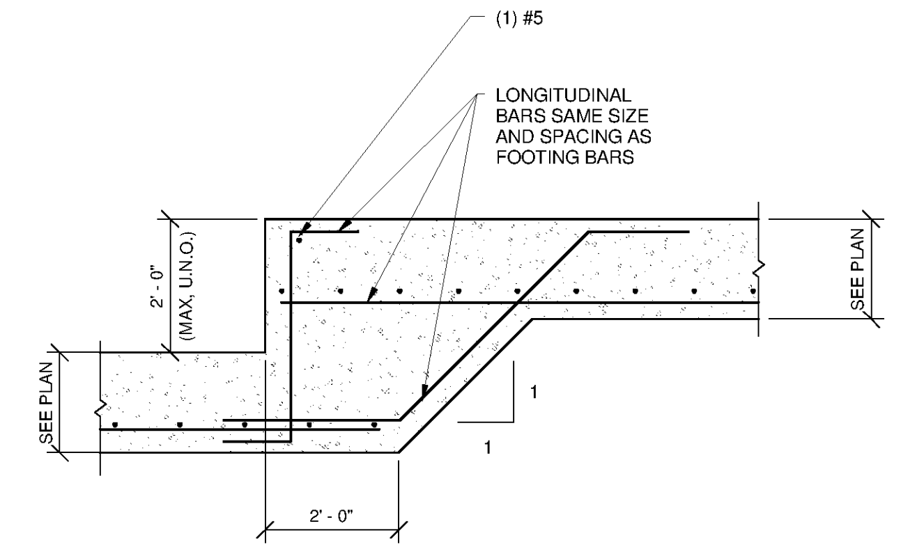
8 STEPPED FOOTING DETAIL SCALE: 1/2" = 1'-0"
