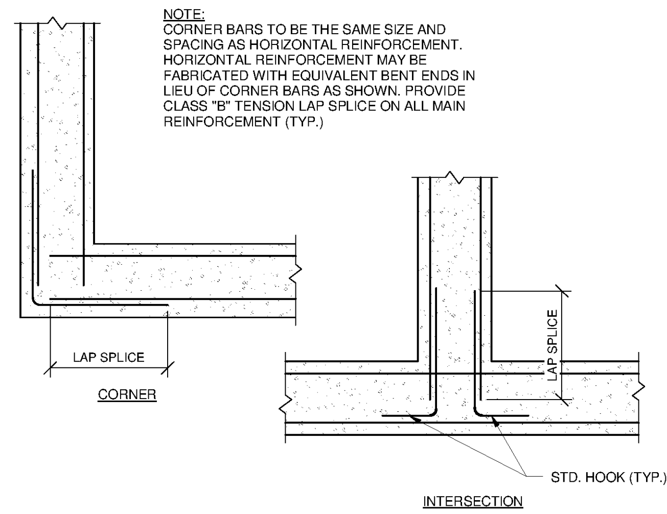
3 WALL CORNERS @ BLDG WALLS SCALE: 3/4" = 1'-0"
