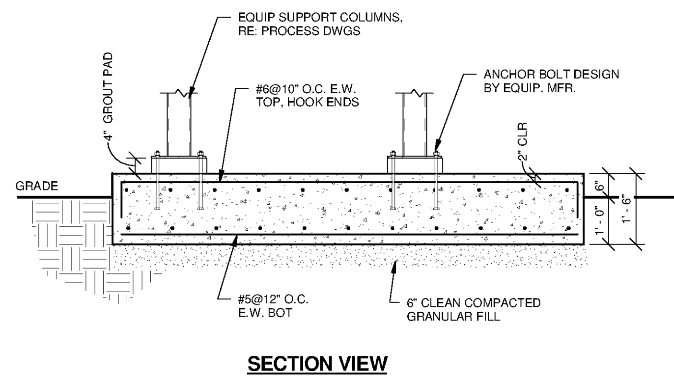
9 PAC EQUIPMENT PAD (1 REQ'D) SCALE: 1/4" = 1'-0"
