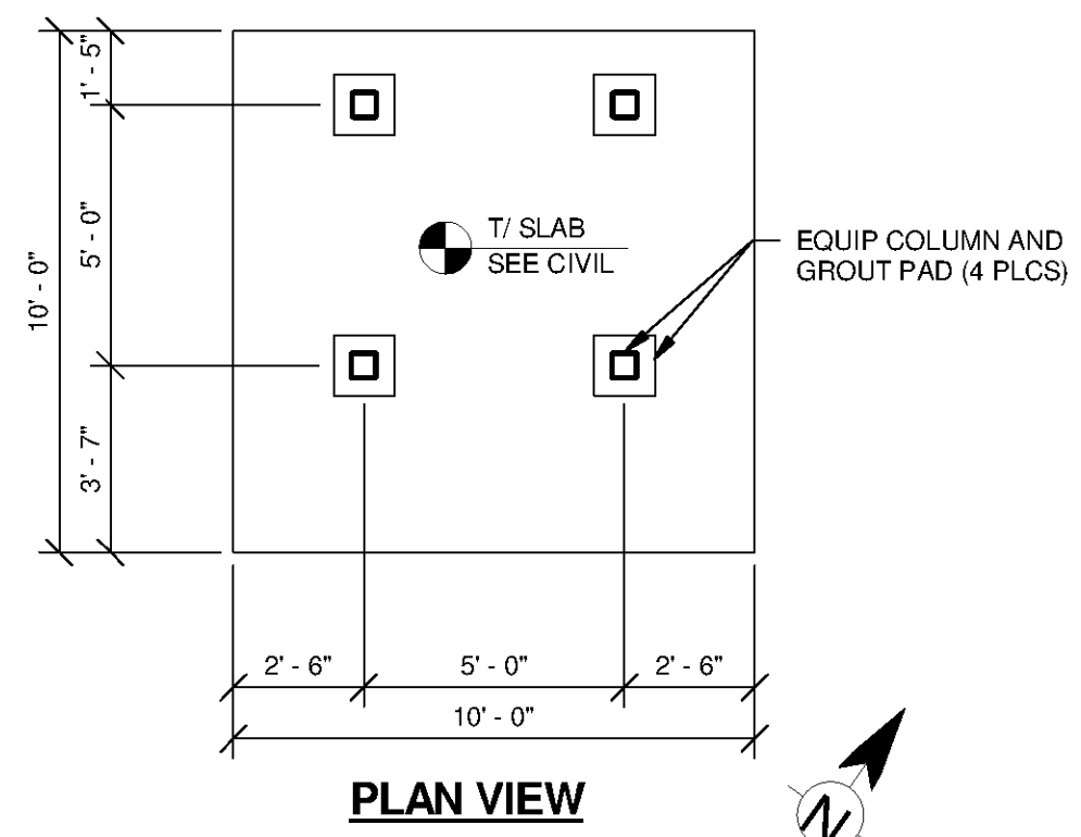
9 PAC EQUIPMENT PAD (1 REQ'D) SCALE: 1/4" = 1'-0"
