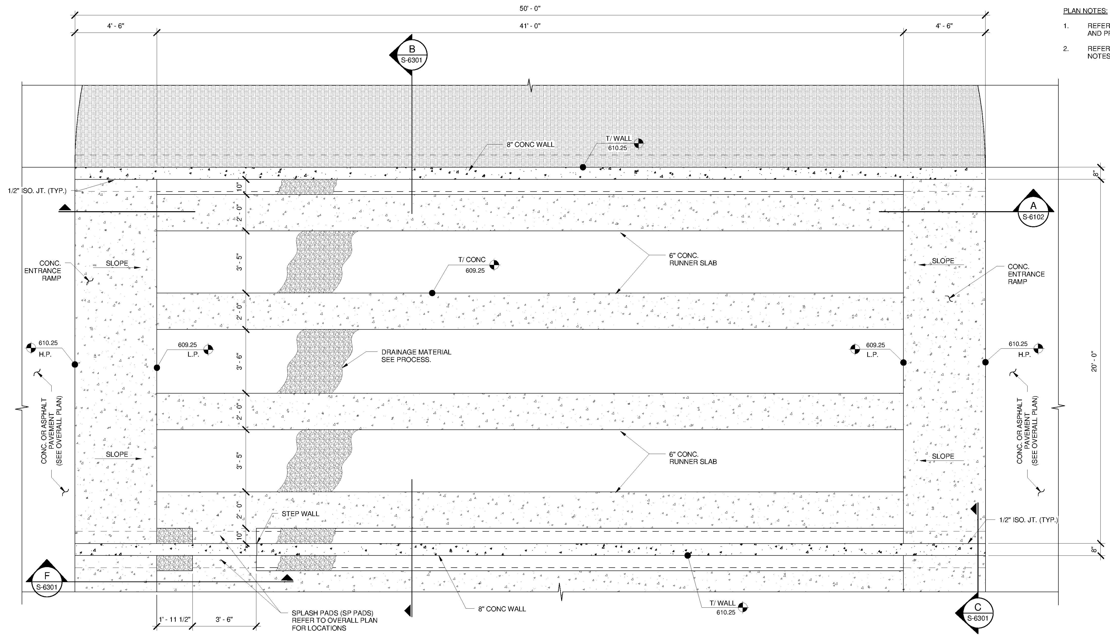
1 DRYING BED ENLARGED PLAN S-6101 SCALE: 3/8" = 1'-0"
