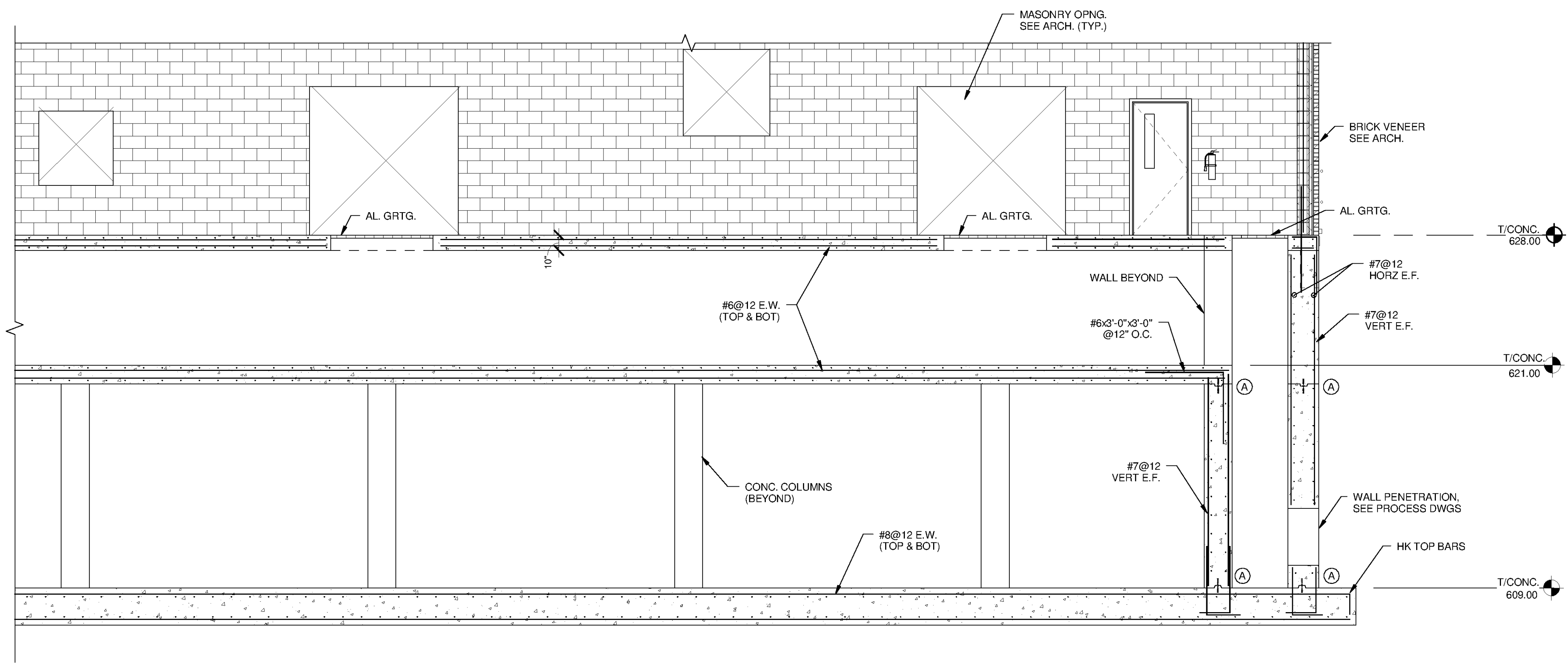
D BUILDING SECTION S-3101 SCALE: 1/4" = 1'-0"
