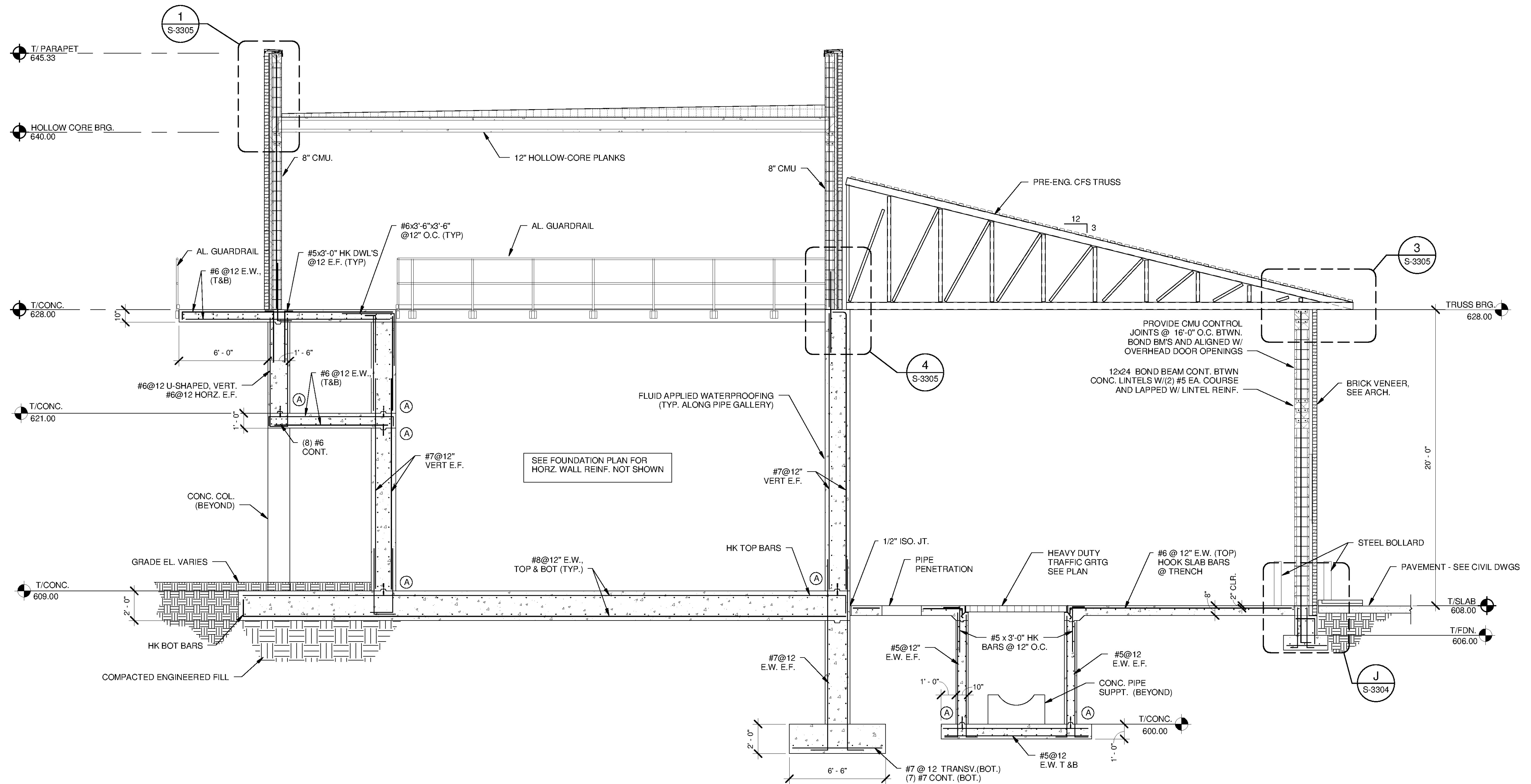
A BUILDING SECTION S-3101 SCALE: 1/4" = 1'-0"
