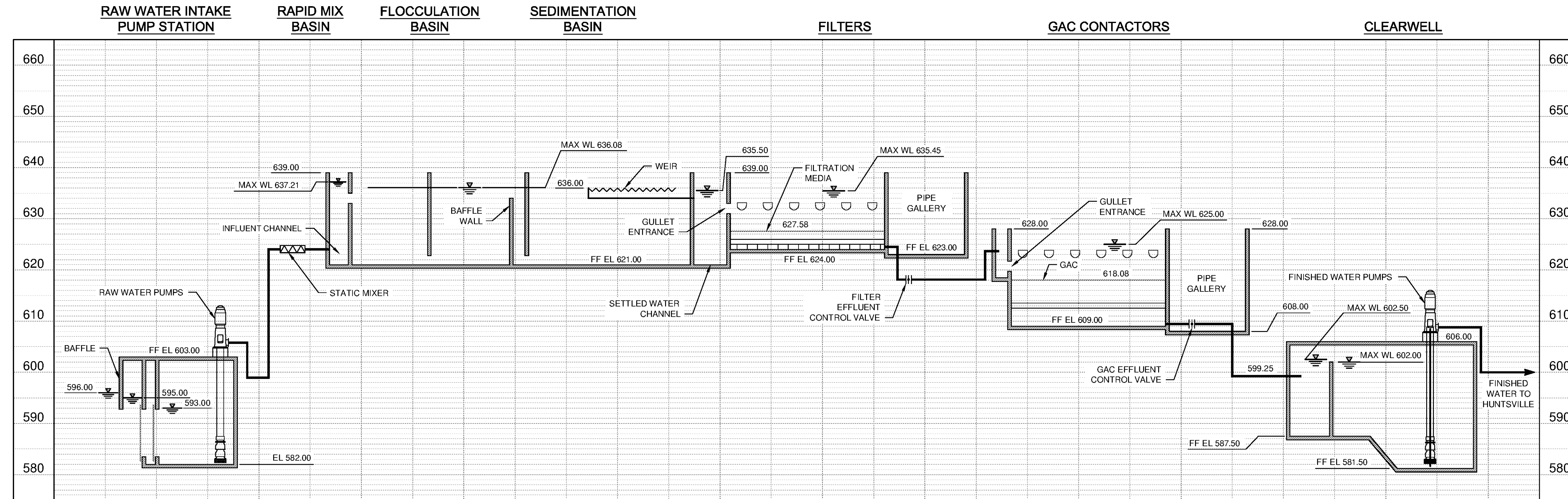
HYDRAULIC PROFILE FOR PROCESS FLOW
