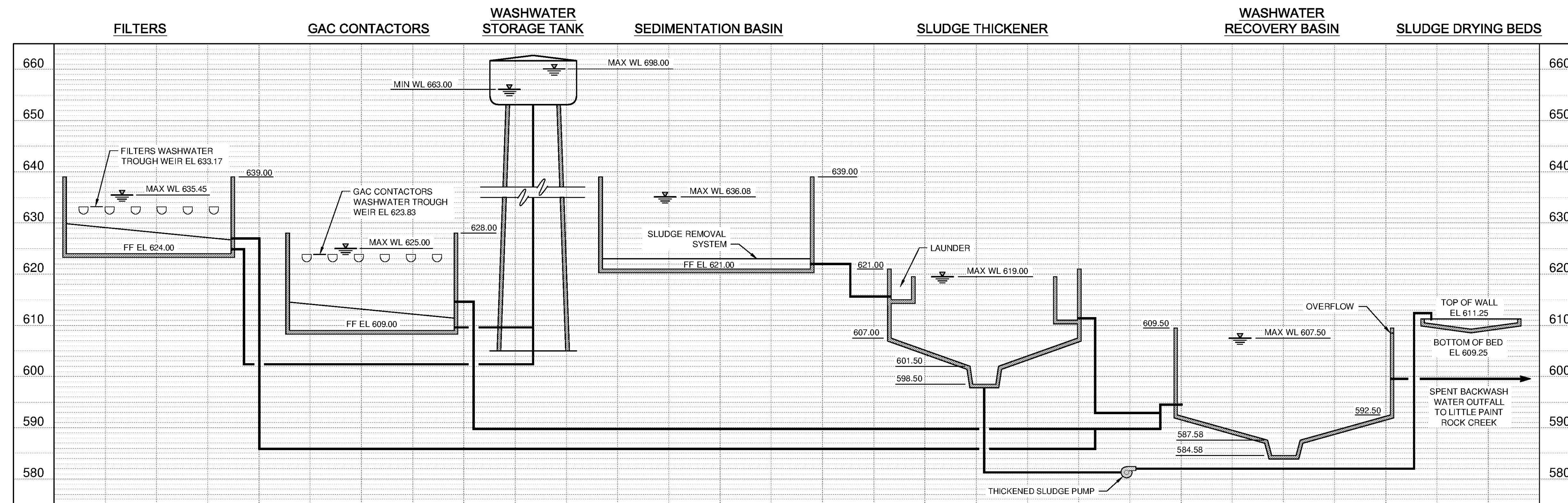
HYDRAULIC PROFILE FOR WASHWATER AND SLUDGE FLOWS
